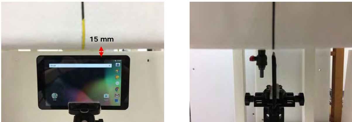
Fig.11 EUT Left side (15mm) to flat phantom
