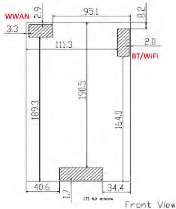
Fig.14 Antenna position of EUT (Front view)
