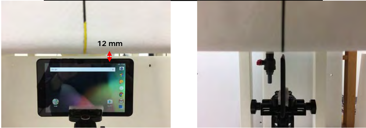
Fig.6 EUT Right side (12mm) to flat phantom
