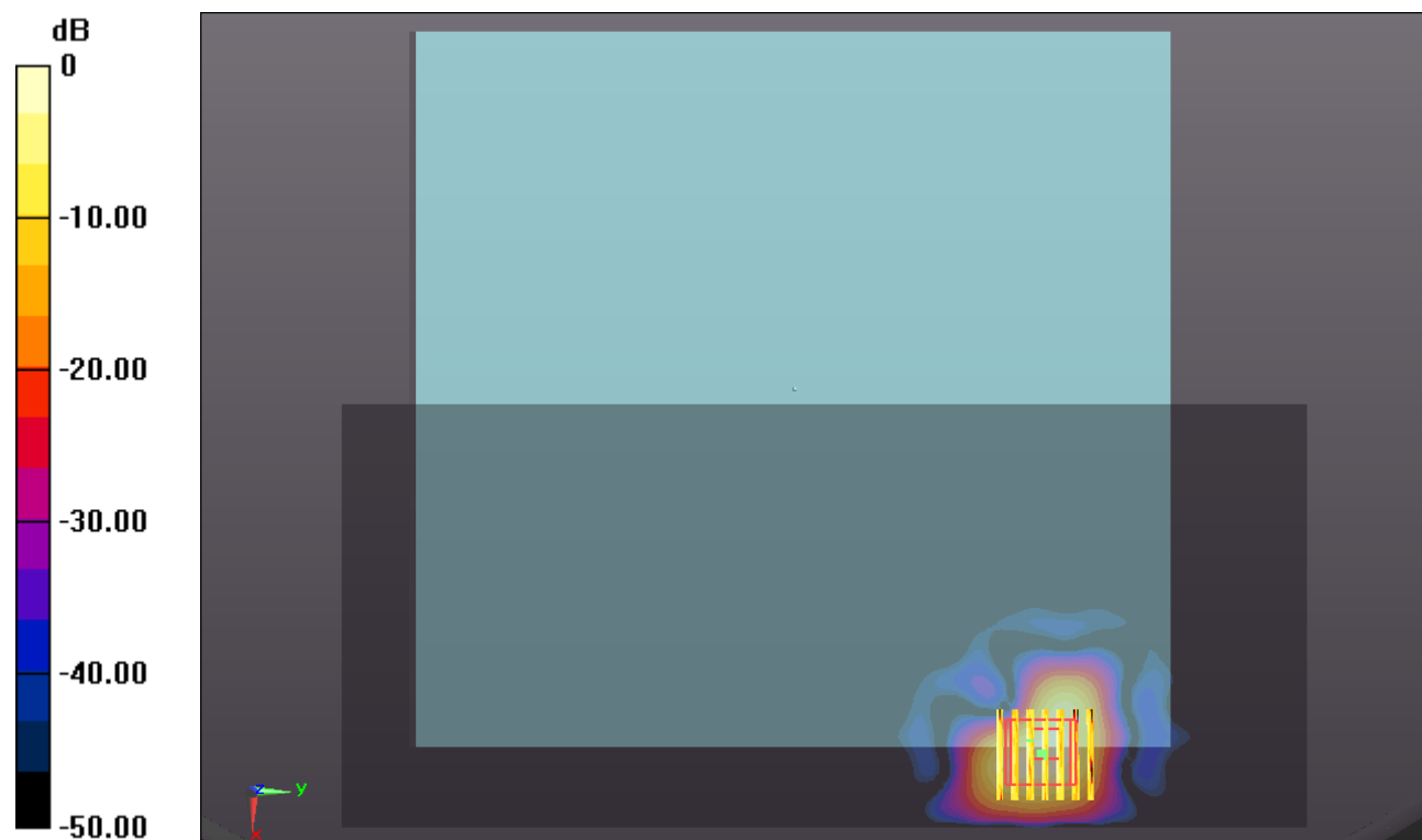
0 dB = 0.020mW/g
