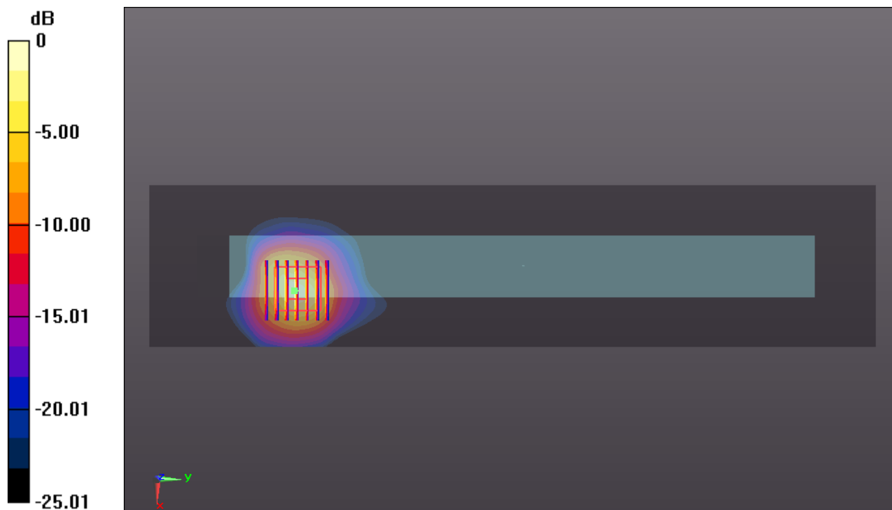
0 dB = 1.370mW/g
