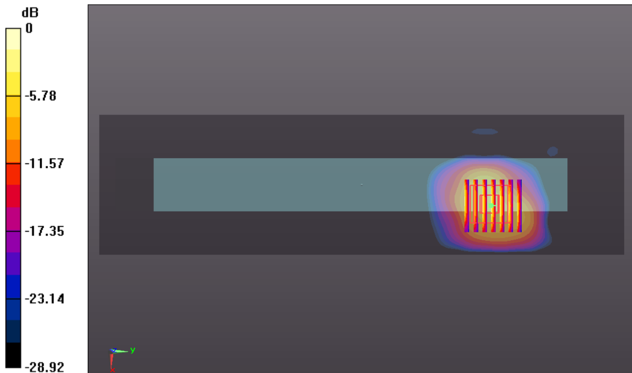
0 dB = 0.690mW/g
