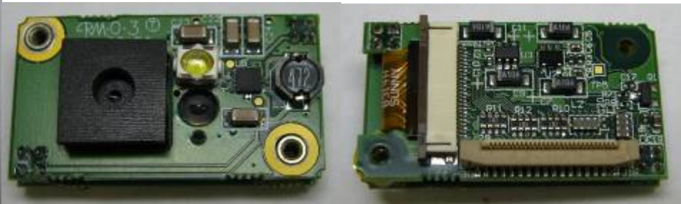
AHL60- CAMERA Top & Bottom ASSY. (8900KM)
