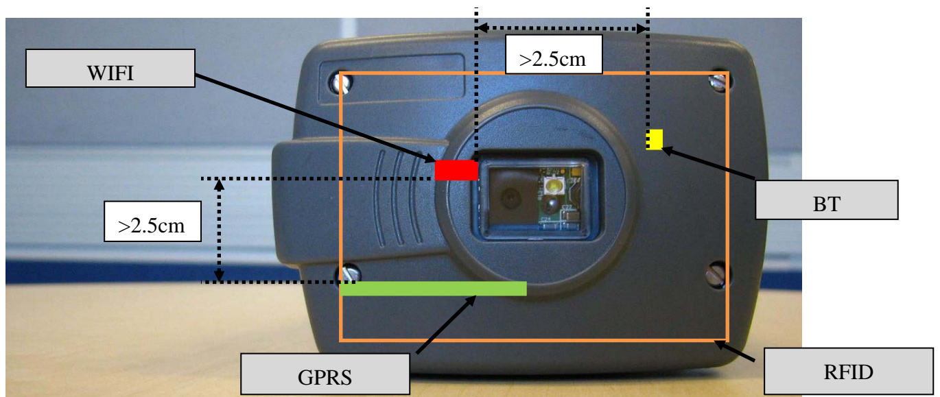
Fig. 19: Top view of the device CE 5240 with antenna diagram.
