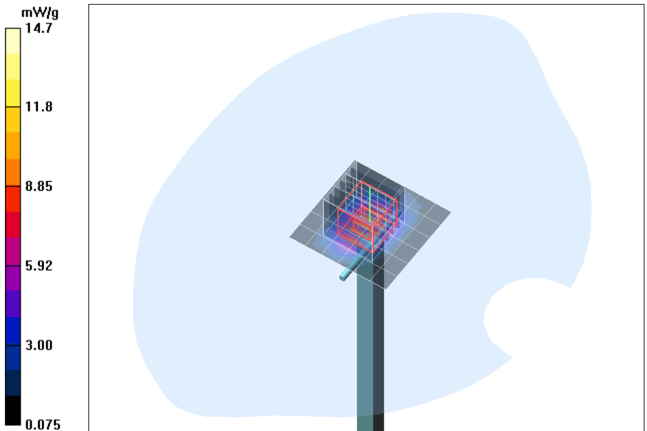
Fig. 13: Validation measurement 2450 MHz Body (December 23. 2009). coarse grid. Ambient Temperature: 20.6°C. Liquid Temperature: 20.2°C.
