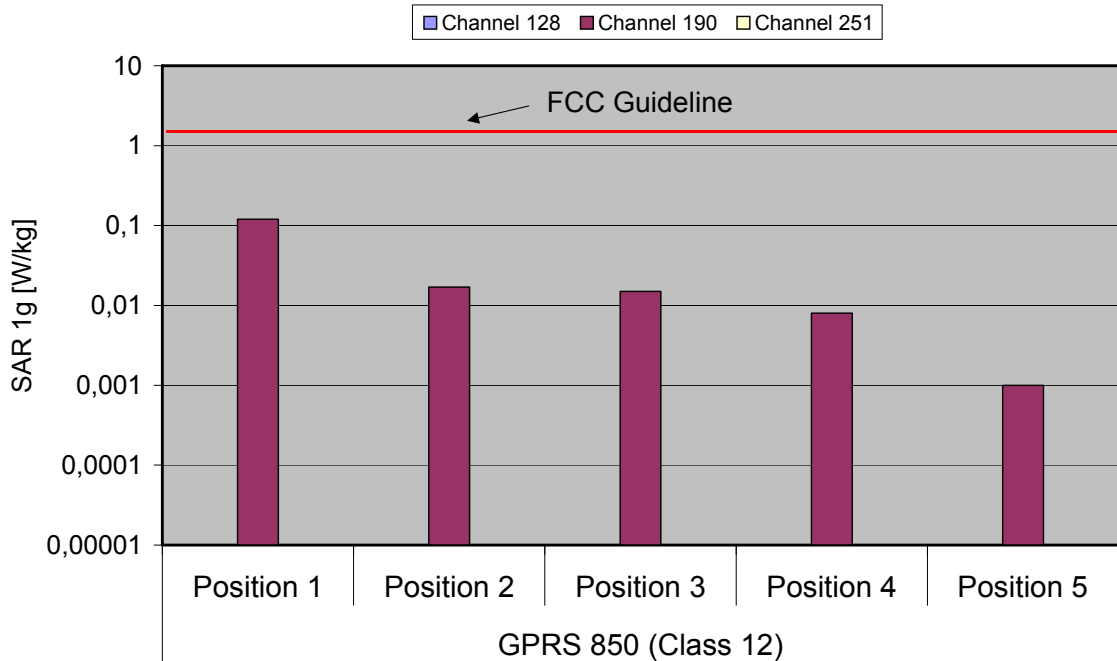
Fig. 8: The measured SAR values for the DAP Technologies CE 5240 for GPRS 850 (Class 12) in comparison to the FCC exposure limit.
