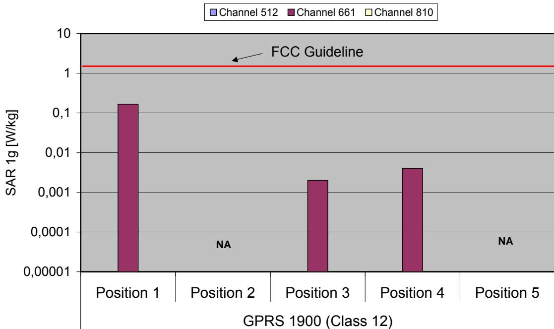
Fig. 9: The measured SAR values for the DAP Technologies CE 5240 for GPRS 1900 (Class 12) in comparison to the FCC exposure limit.
