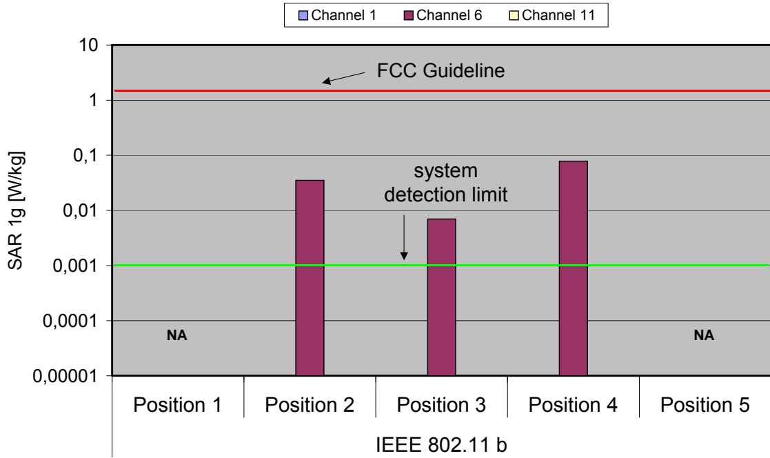
Fig. 10: The measured SAR values for the DAP Technologies CE 5240 for IEEE 802.11 b in comparison to the FCC exposure limit.
