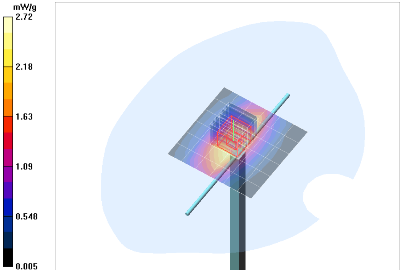
Fig. 11: Validation measurement 835 MHz Body (December 14. 2009). coarse grid. Ambient Temperature: 20.6°C. Liquid Temperature: 20.4°C.
