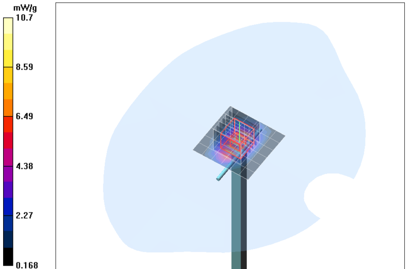
Fig. 12: Validation measurement 1900 MHz Body (December 11. 2009). coarse grid. Ambient Temperature: 21.3°C. Liquid Temperature: 20.9°C.
