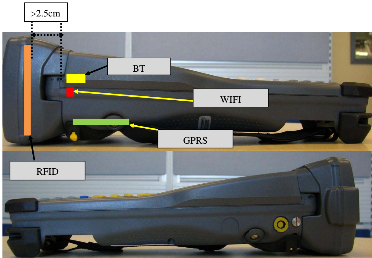
Fig. 18: Side view of the device CE 5240 with antenna diagram.
