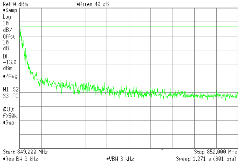
Plot 7.4.2) GSMK; Cellular high channel, above 849 MHz
