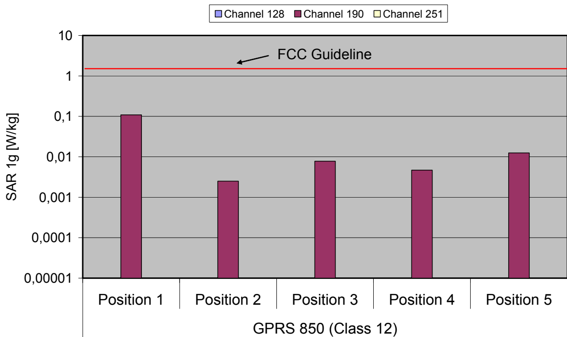
Fig. 8: The measured SAR values for the DAP Technologies 5000B1 for GPRS 850 (Class 12) in comparison to the FCC exposure limit.
