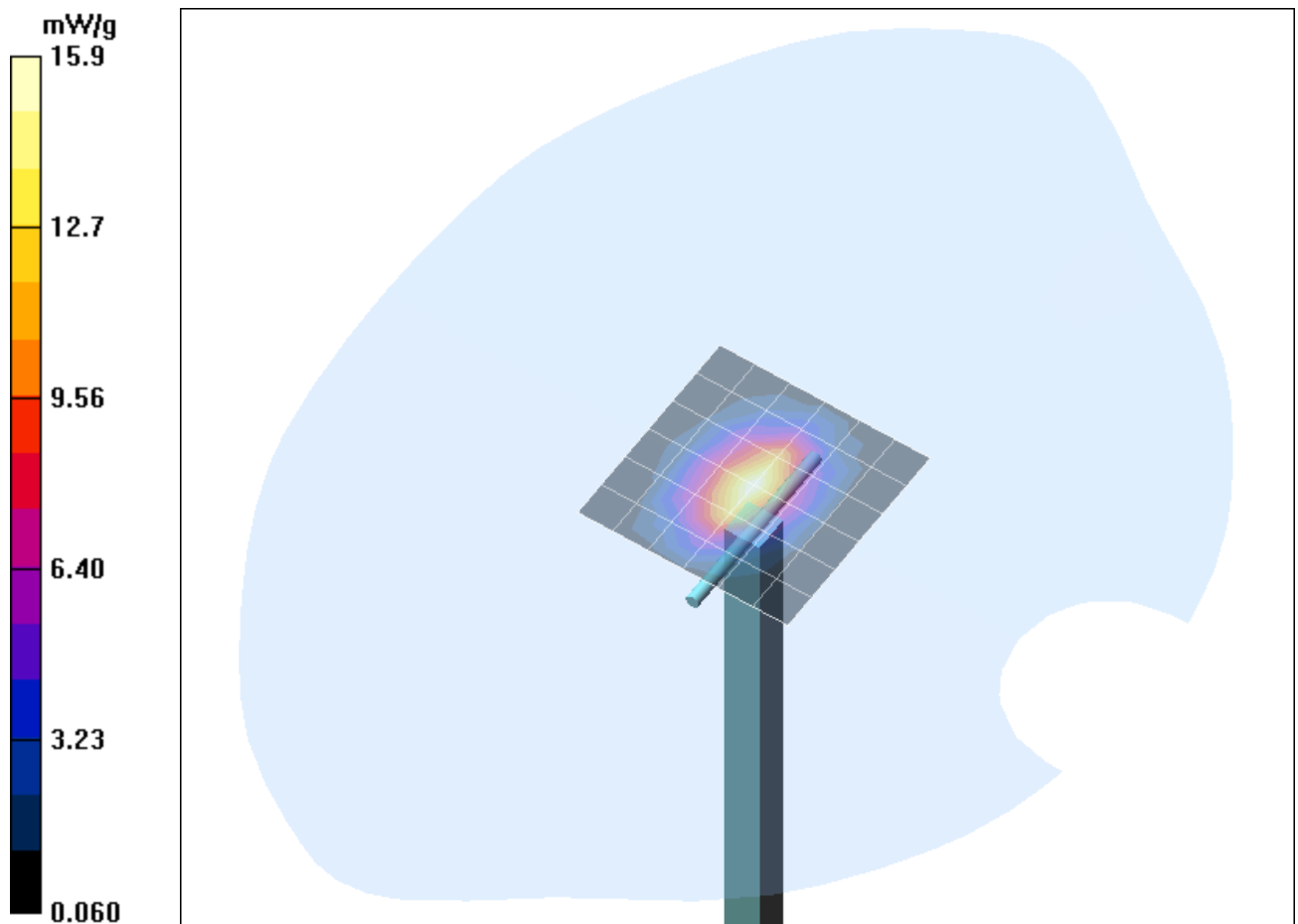
Fig. 13: Validation measurement 2450 MHz Body (March 31, 2009), coarse grid. Ambient Temperature: 22.1°C, Liquid Temperature: 21.4°C.
