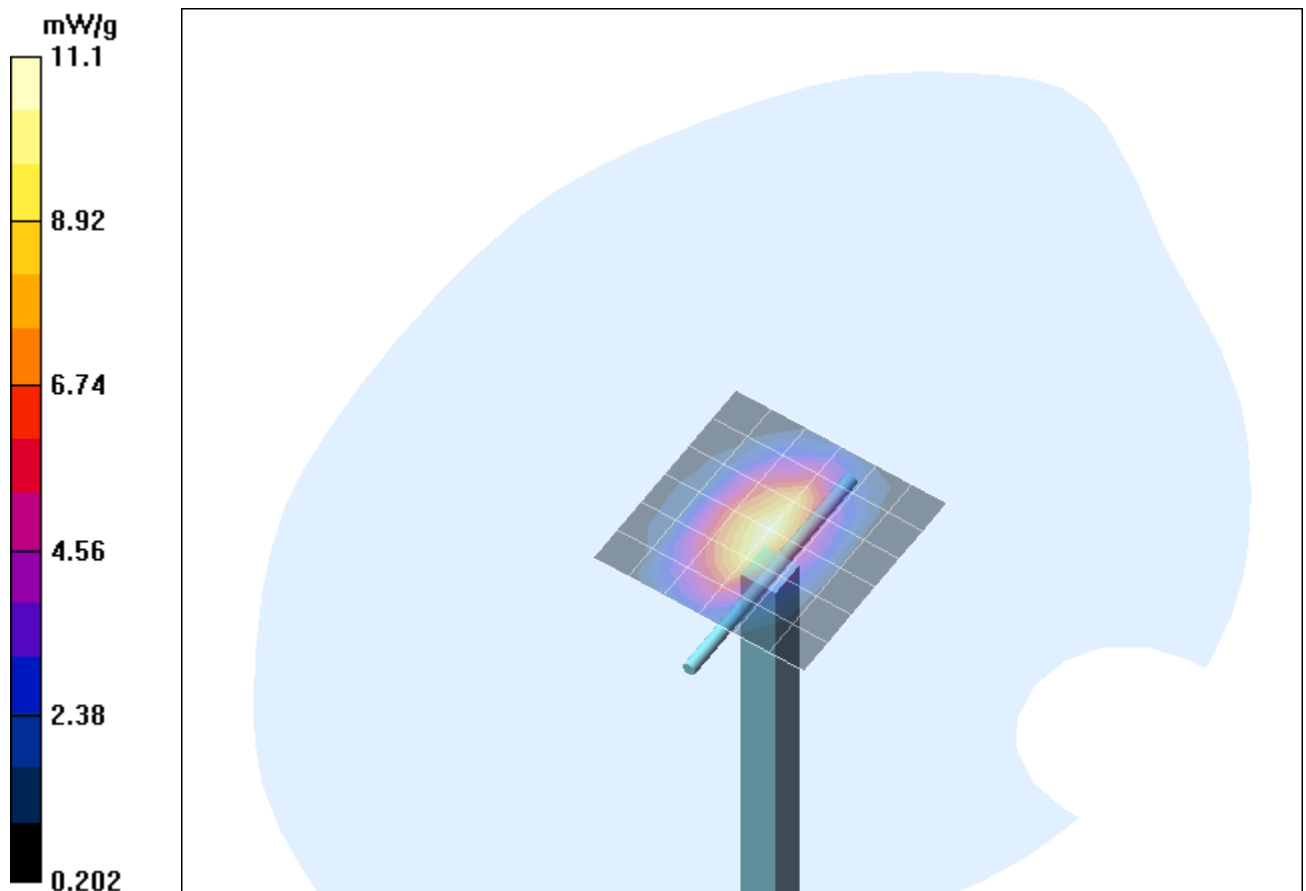
Fig. 12: Validation measurement 1900 MHz Body (April 06, 2009), coarse grid. Ambient Temperature: 22.7°C, Liquid Temperature: 21.6°C.
