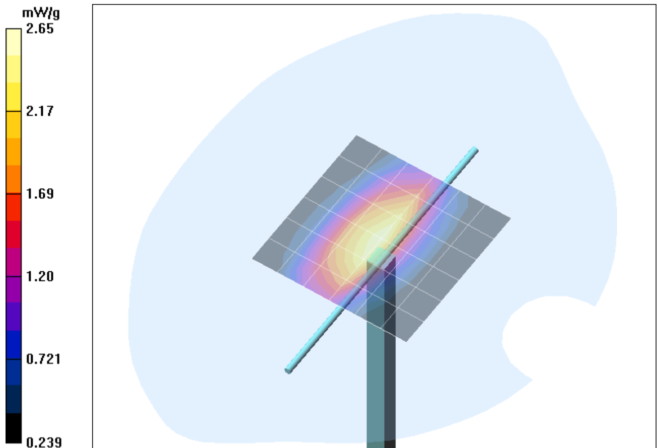
Fig. 11: Validation measurement 835 MHz Body (April 07, 2009), coarse grid. Ambient Temperature: 22.3°C, Liquid Temperature: 21.5°C.
