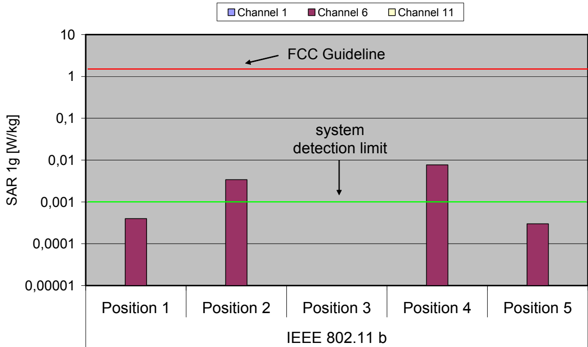
Fig. 10: The measured SAR values for the DAP Technologies 5000B1 for IEEE 802.11 b in comparison to the FCC exposure limit.
