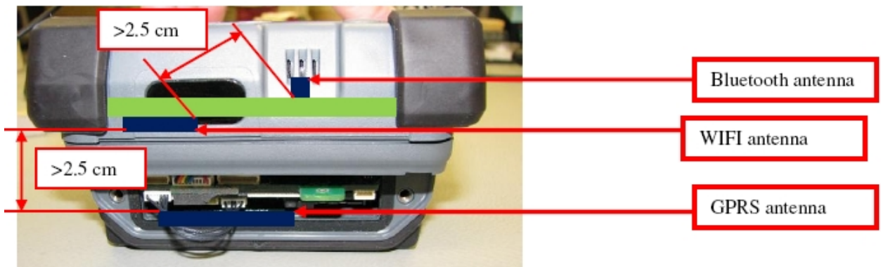
Fig. 17: Top view of the device 5000B1 with antenna diagram.
