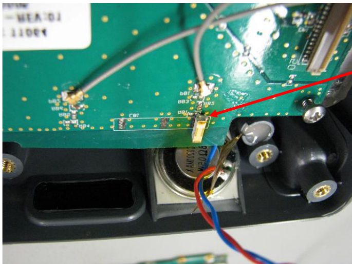
Bluetooth antenna view
