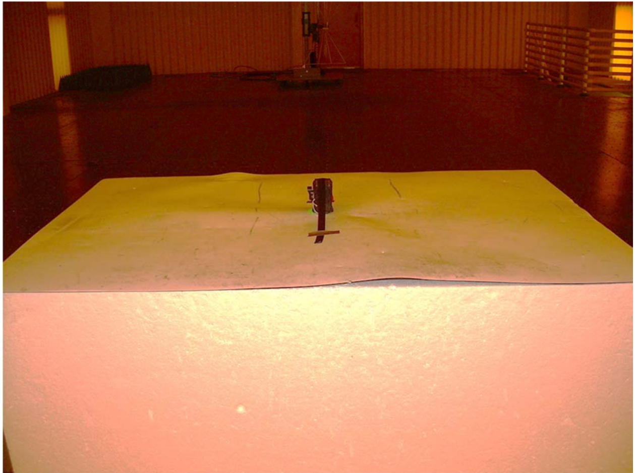
Back View Radiated Emission Test Set Up – Vertical Configuration
