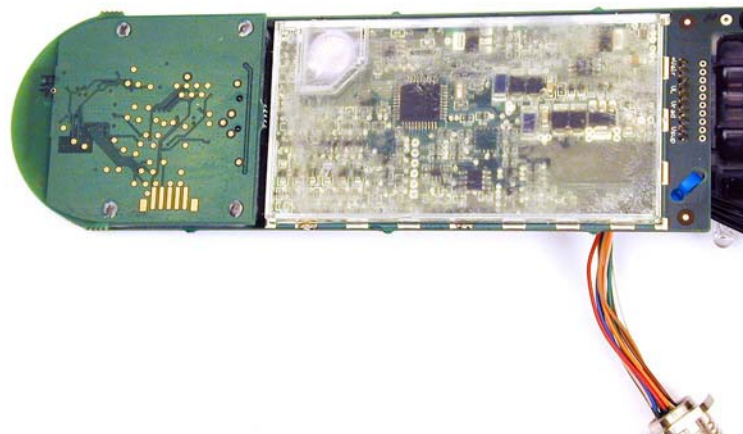
SE7SensBd04
