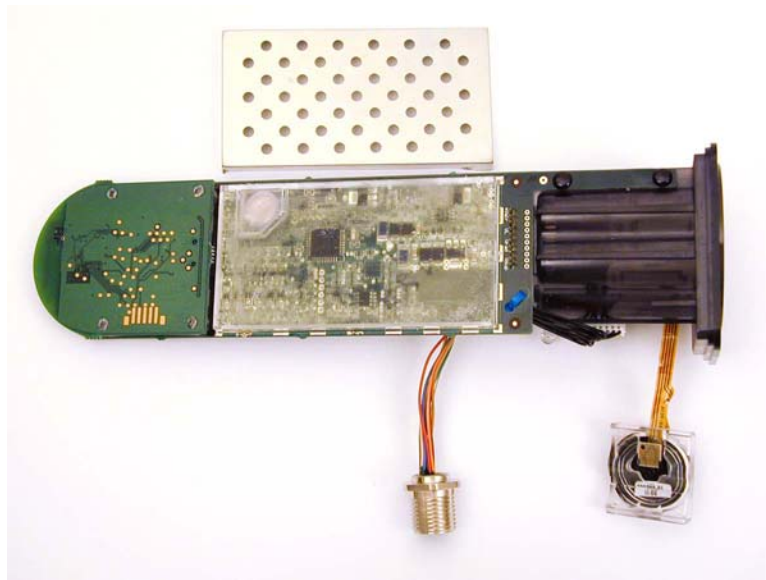
SE7SensBd03
