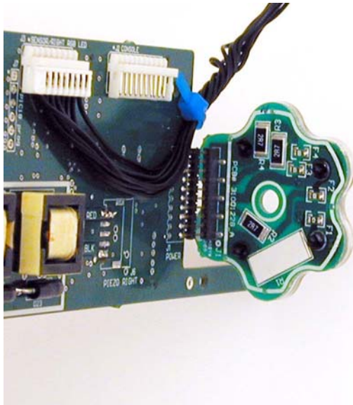
SE7SensBdBattBd01
