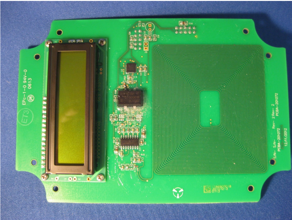
Front of board with RFID section
