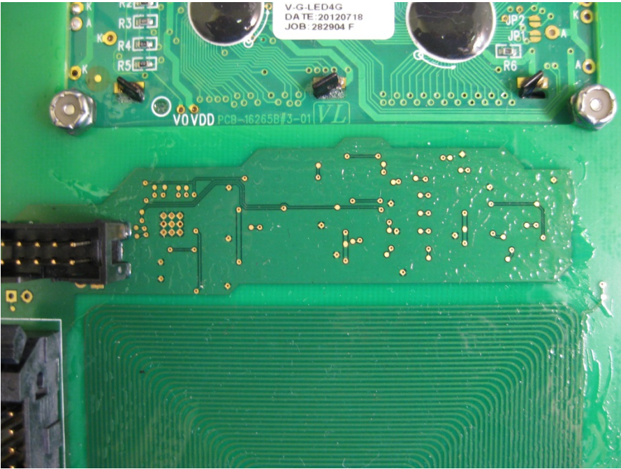
Close up of back side RFID section
