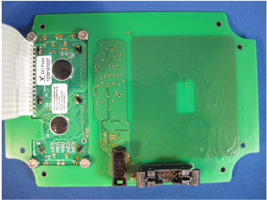
Back of board with RFID section
