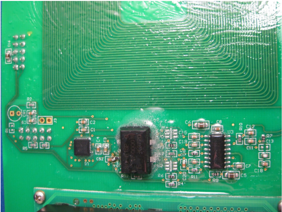
Close up of front side RFID section
