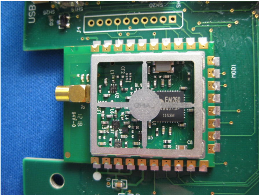
Close up of Apex LT module with shield removed
