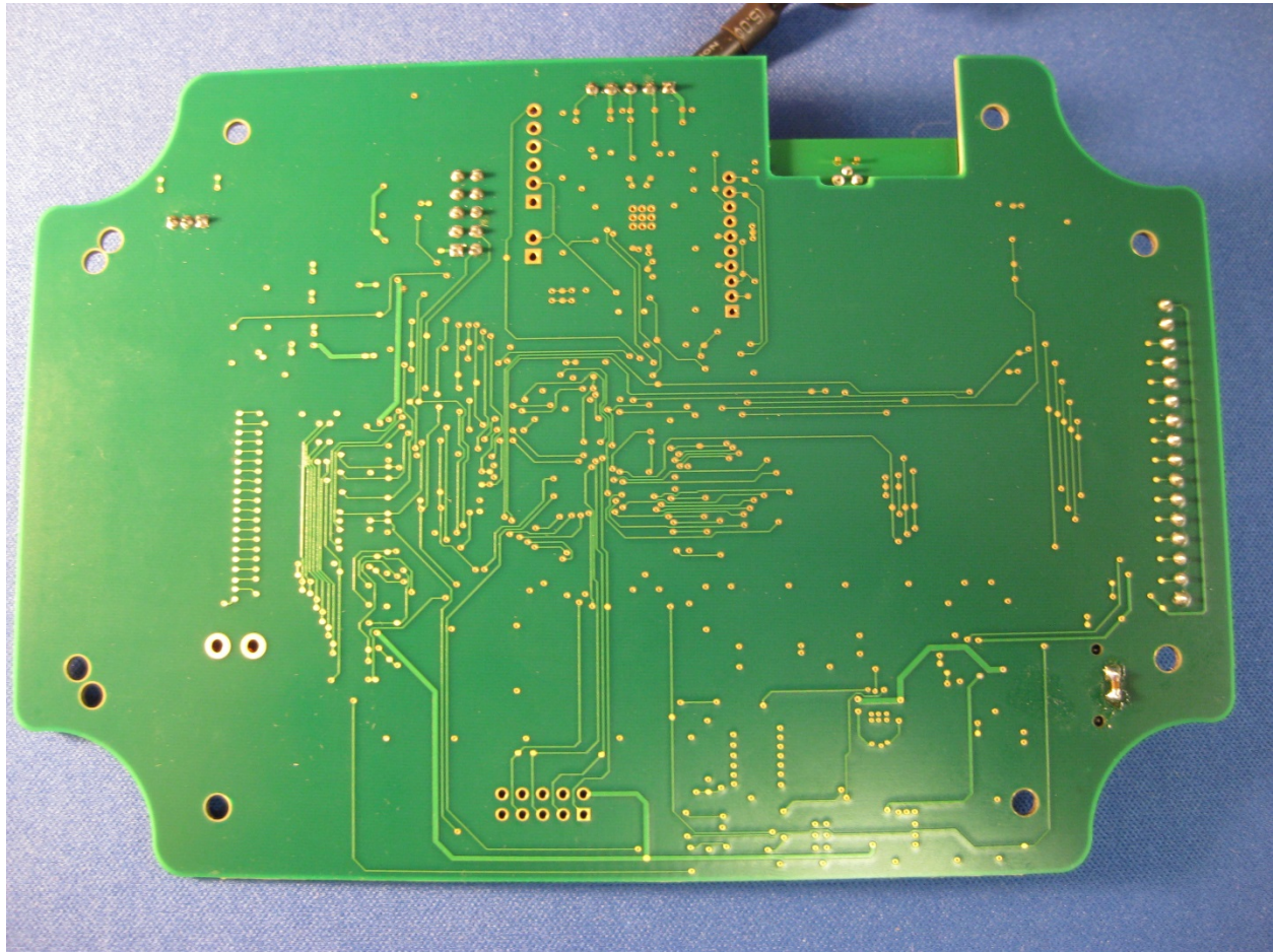
Back side of board with Apex LT module
