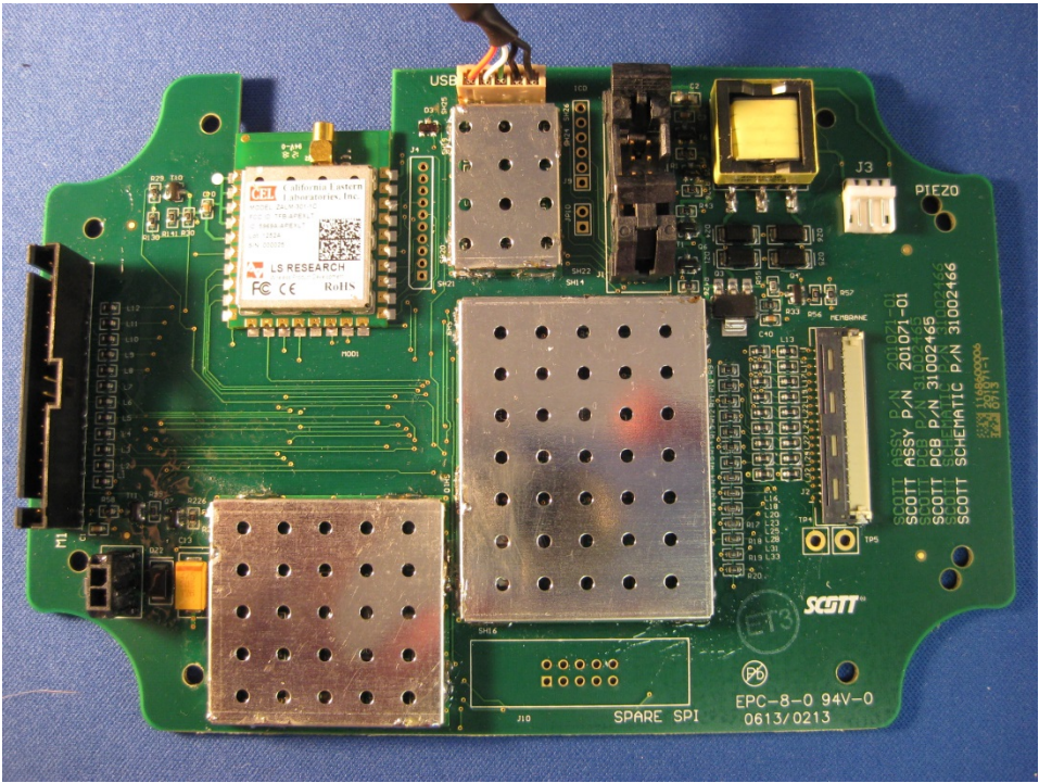
Front side of board with Apex LT Module
