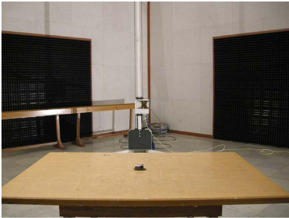
< RADIATED EMISSION SETUP PHOTOGRAPH – FRONT VIEW2 >
