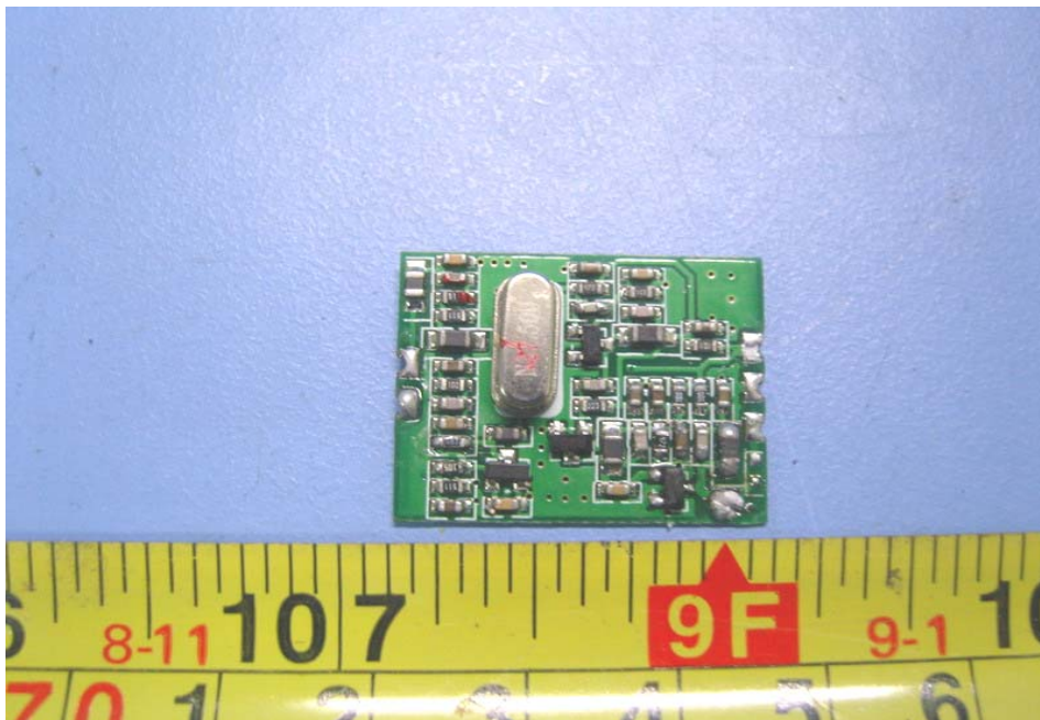
PCB2 - Front View
