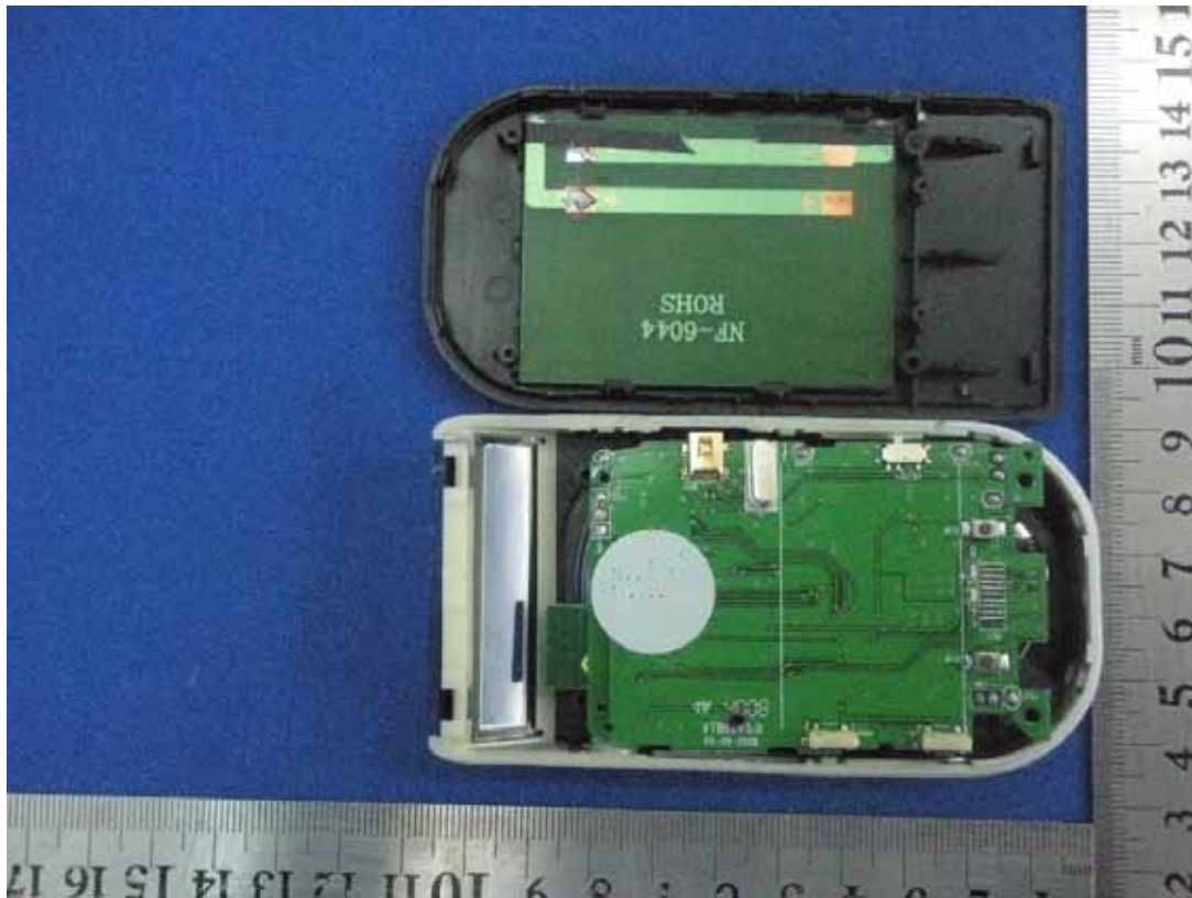
Photo 1 General Appearance of the EUT(Inside)
