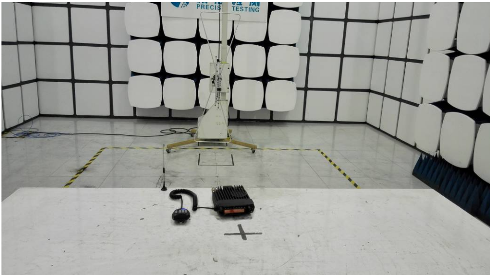
RADIATED EMISSION TEST SETUP BELOW 1GHz
