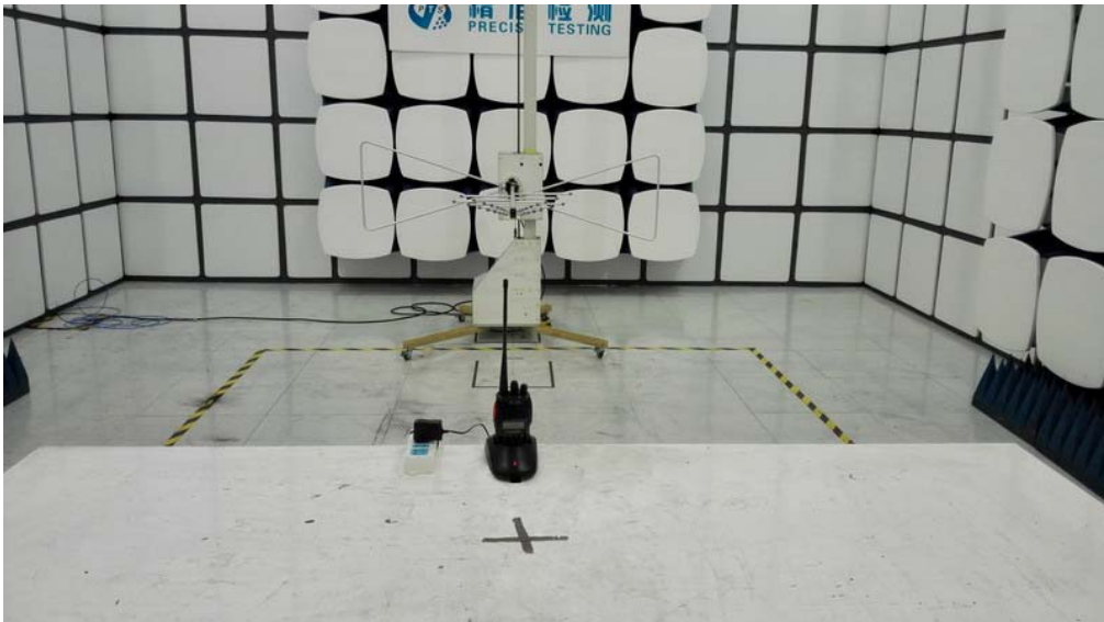
RADIATED EMISSION BELOW 1GHz TEST SETUP
