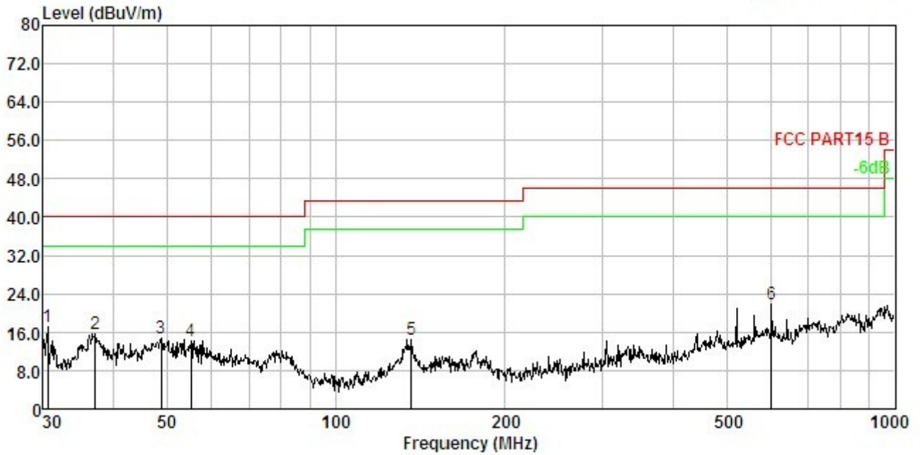
Radiated Emission Test –Horizontal -3m
