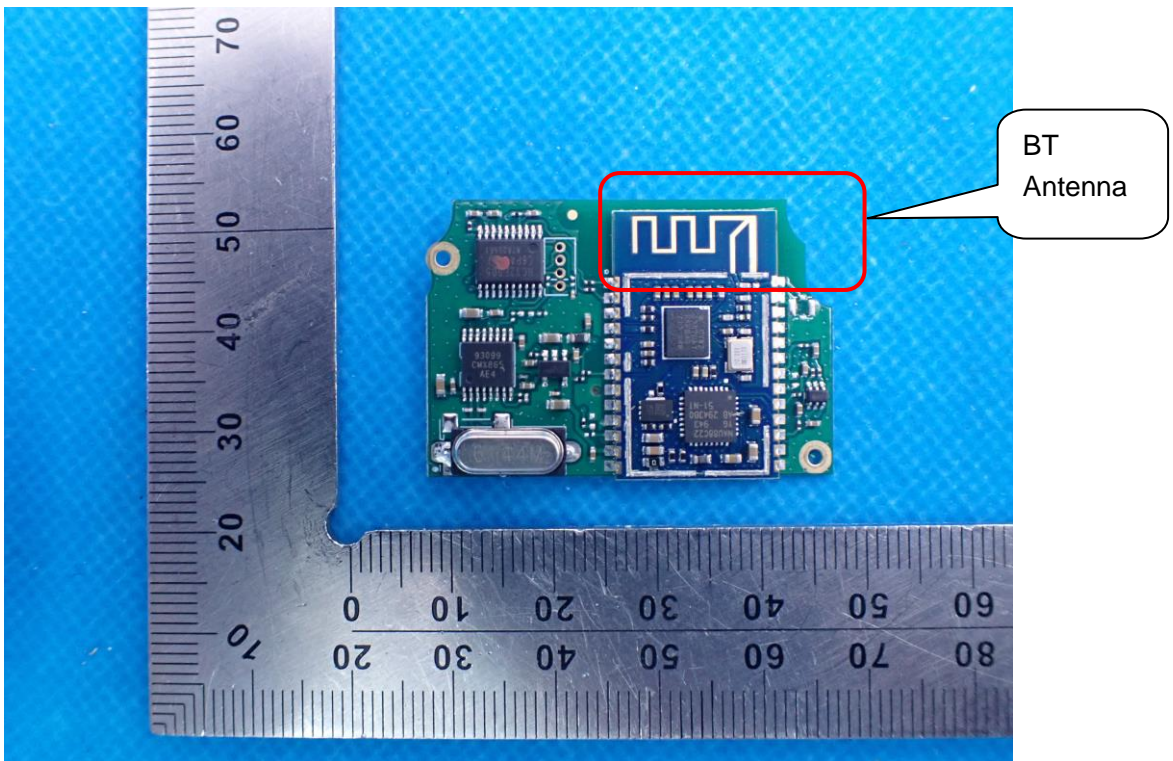
INTERNAL VIEW-8 OF EUT
