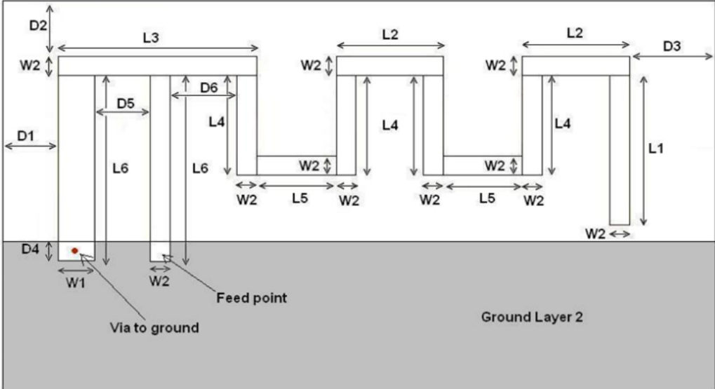
Antenna Dimension
