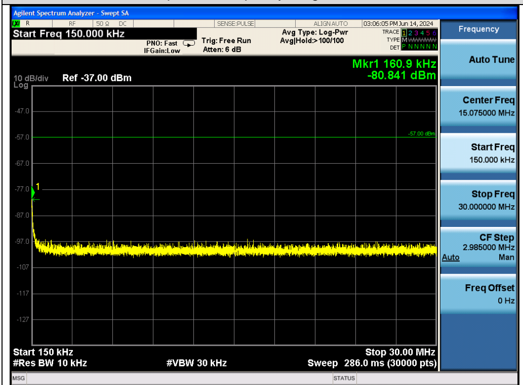
Test_Graph_RX_FrequencyRange_150kHz-30MHz
