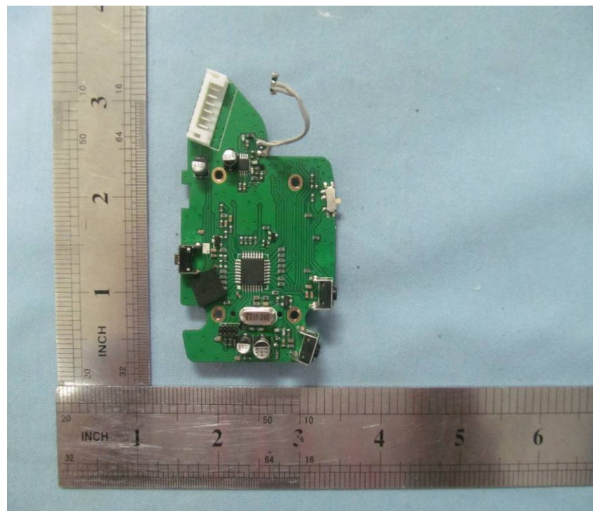
INTERNAL VIEW OF EUT - 7
