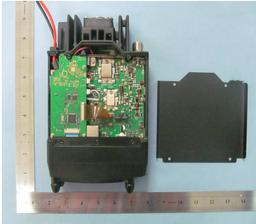
OPEN VIEW2 OF EUT
