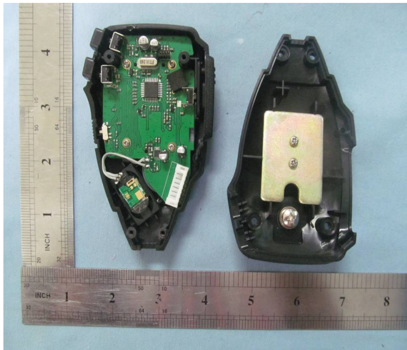
INTERNAL VIEW OF EUT – 1
