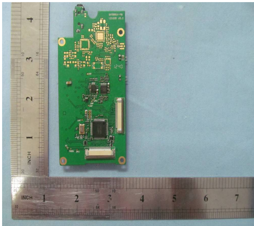
INTERNAL VIEW OF EUT – 1
