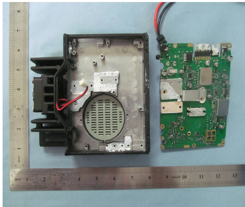
OPEN VIEW2 OF EUT
