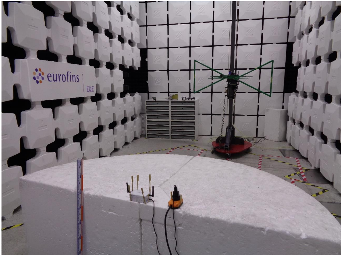
Radiated tests 30MHz to 1GHz USB powered
