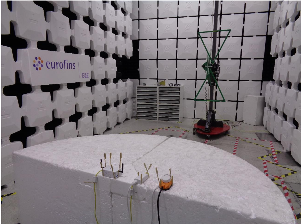
Radiated tests 30MHz to 1GHz PoE powered
