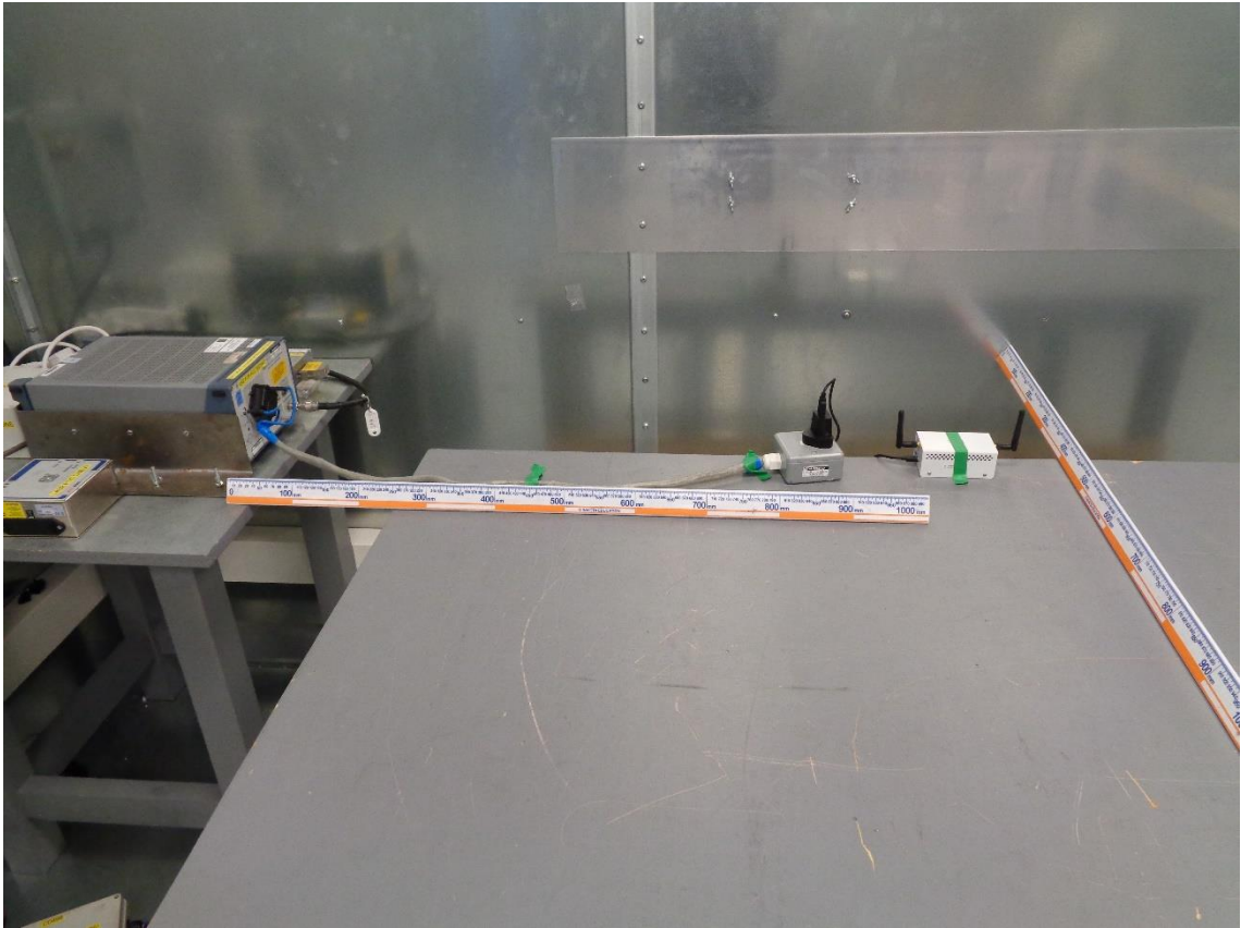
Conducted tests 150kHz-30MHz USB powered
