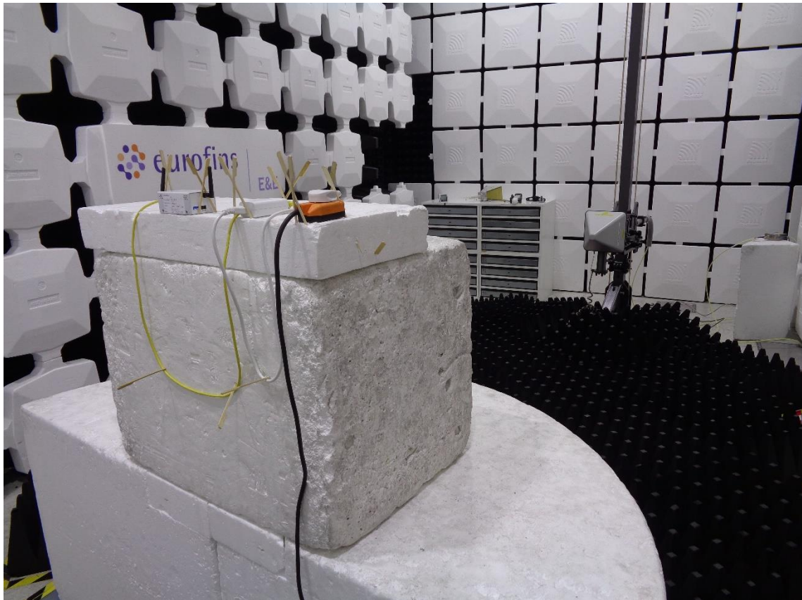
Radiated tests 1-18GHz PoE powered
