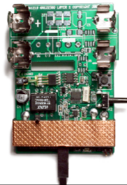
Interior top under antenna
