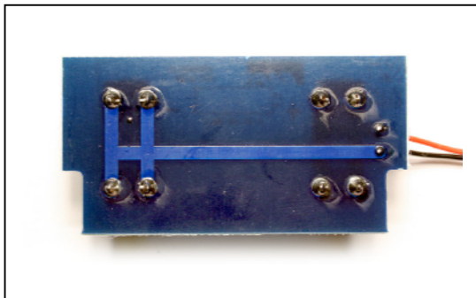
Battery Board Bottom
