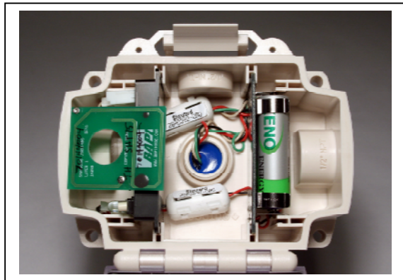
Interior assembly
