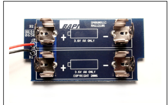
Battery Board Top
