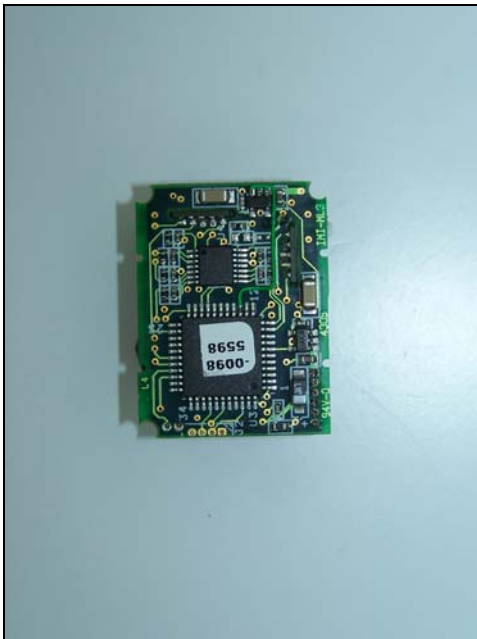
Internal View of EUT – 11
