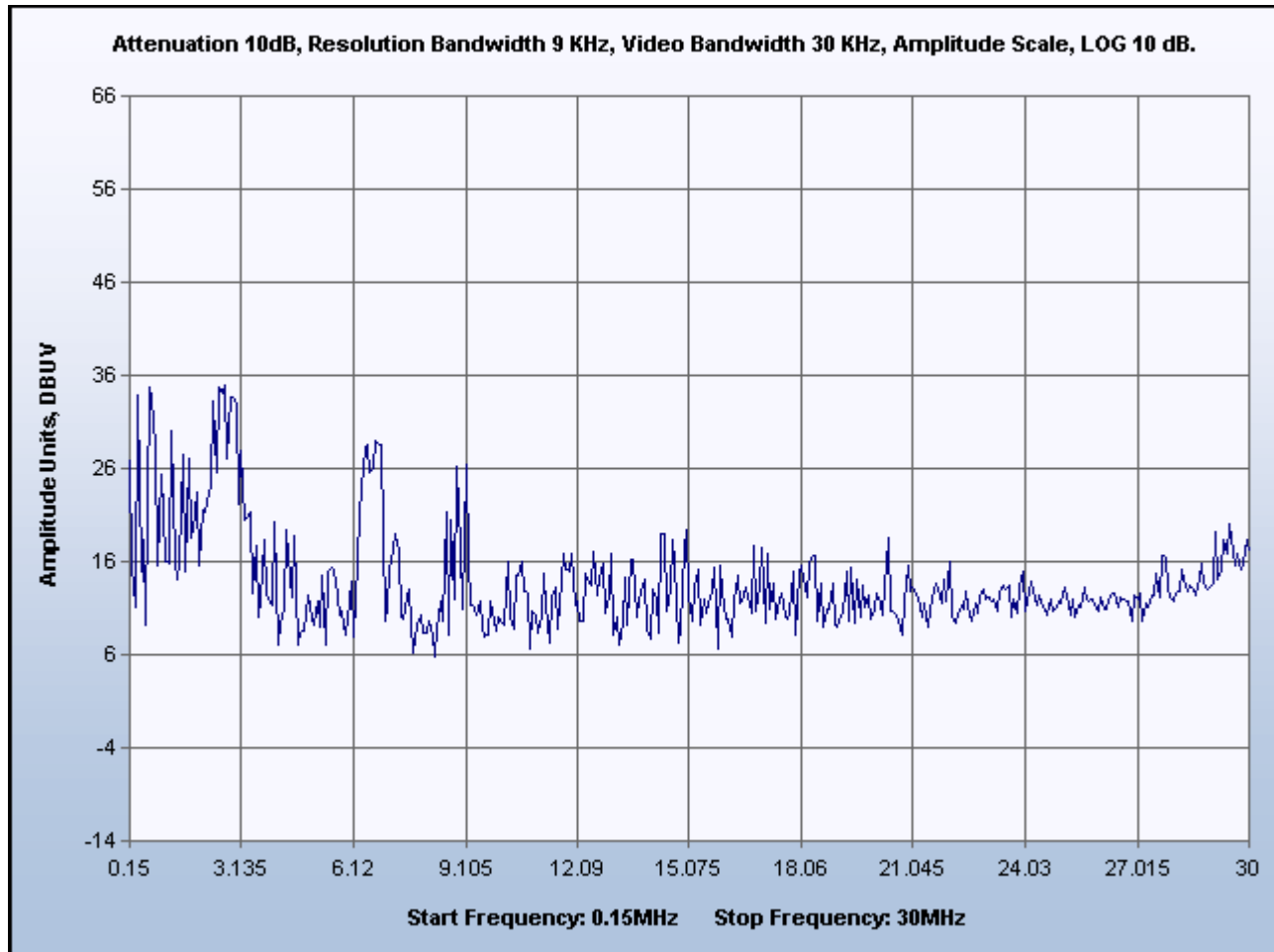
Plot 4. Conducted Emissions, Neutral Line, 0.15 MHz to 30 MHz
