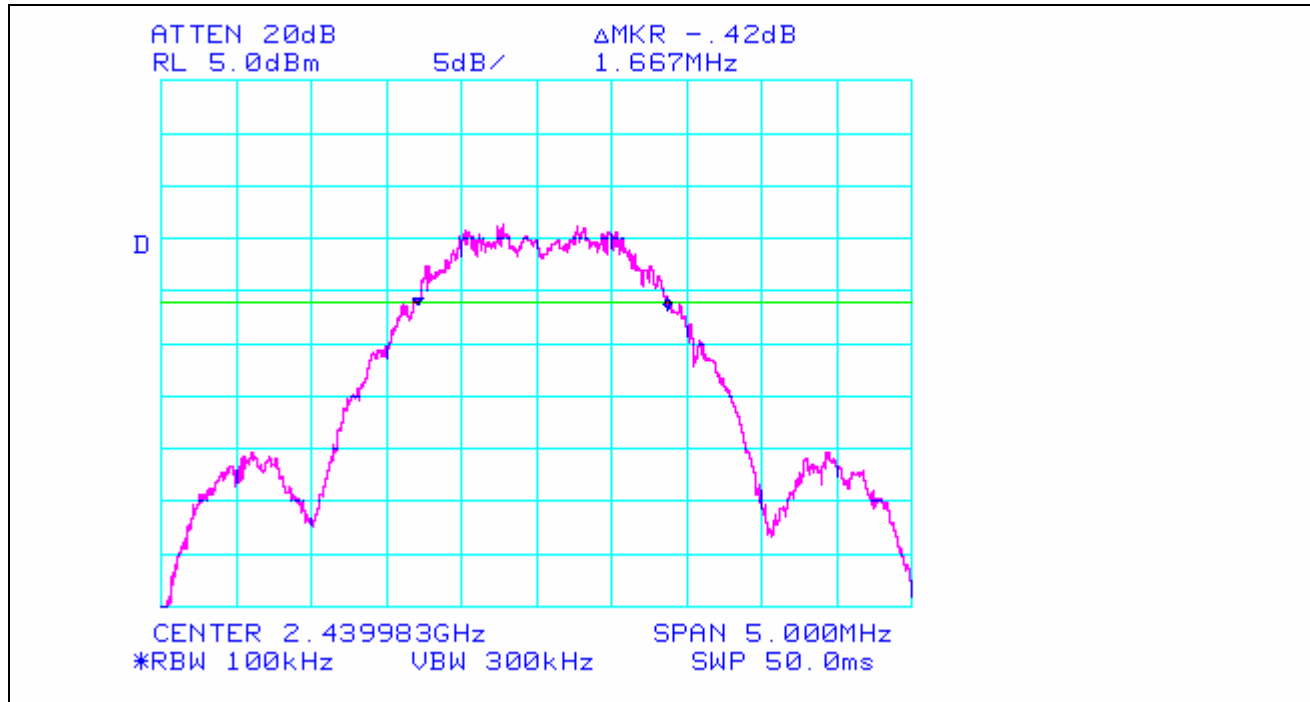
Plot 6. Occupied Bandwidth Test Results – Channel 7
