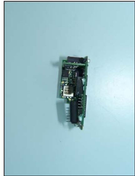
Internal View of EUT - 10
