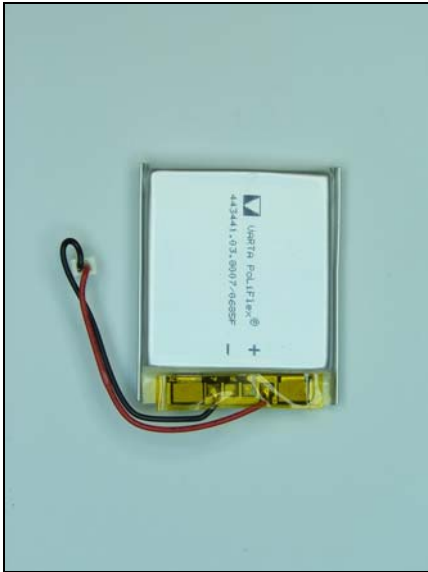
Internal View of EUT – 5
