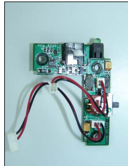
Internal View of EUT – 16
