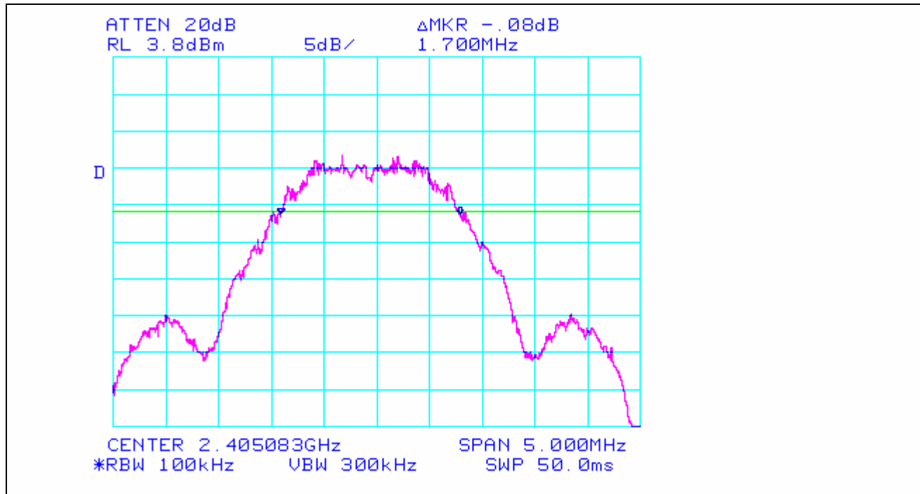
Plot 5. Occupied Bandwidth Test Results – Channel 0
