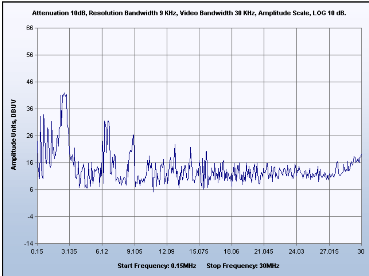
Plot 3. Conducted Emissions, Phase Line, 0.15 MHz to 30 MHz
