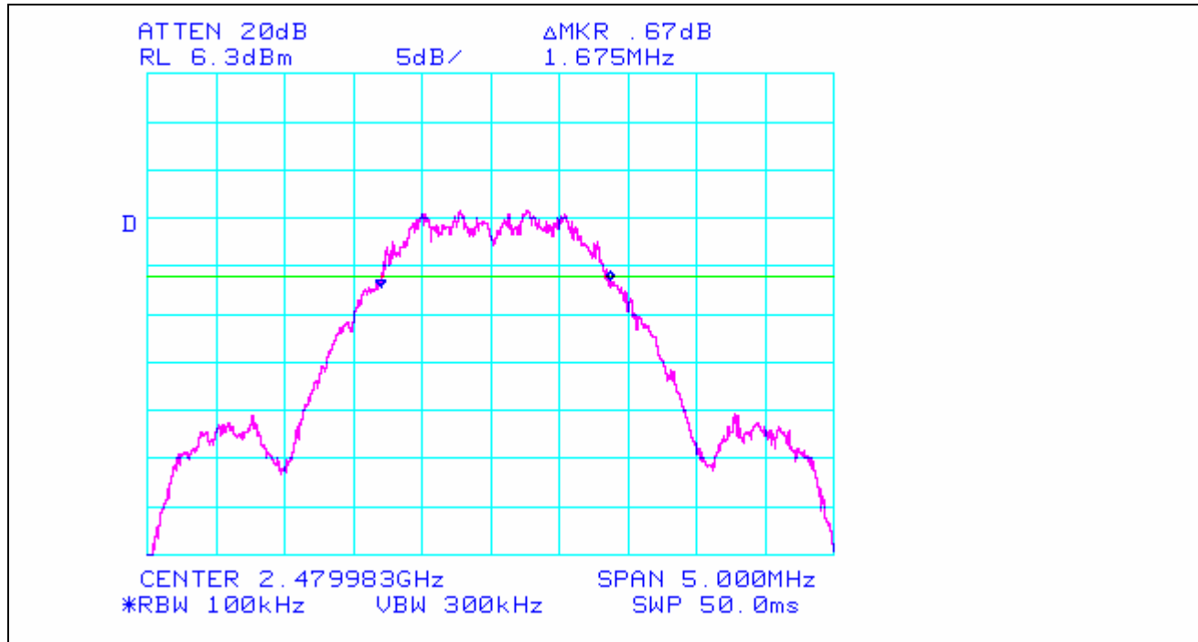
Plot 7. Occupied Bandwidth Test Results – Channel 15
