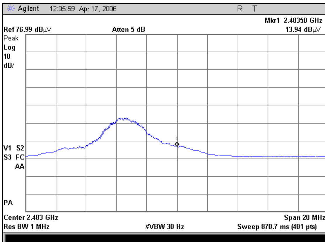
Plot 12. Band Width Emissions Test Results, 2
