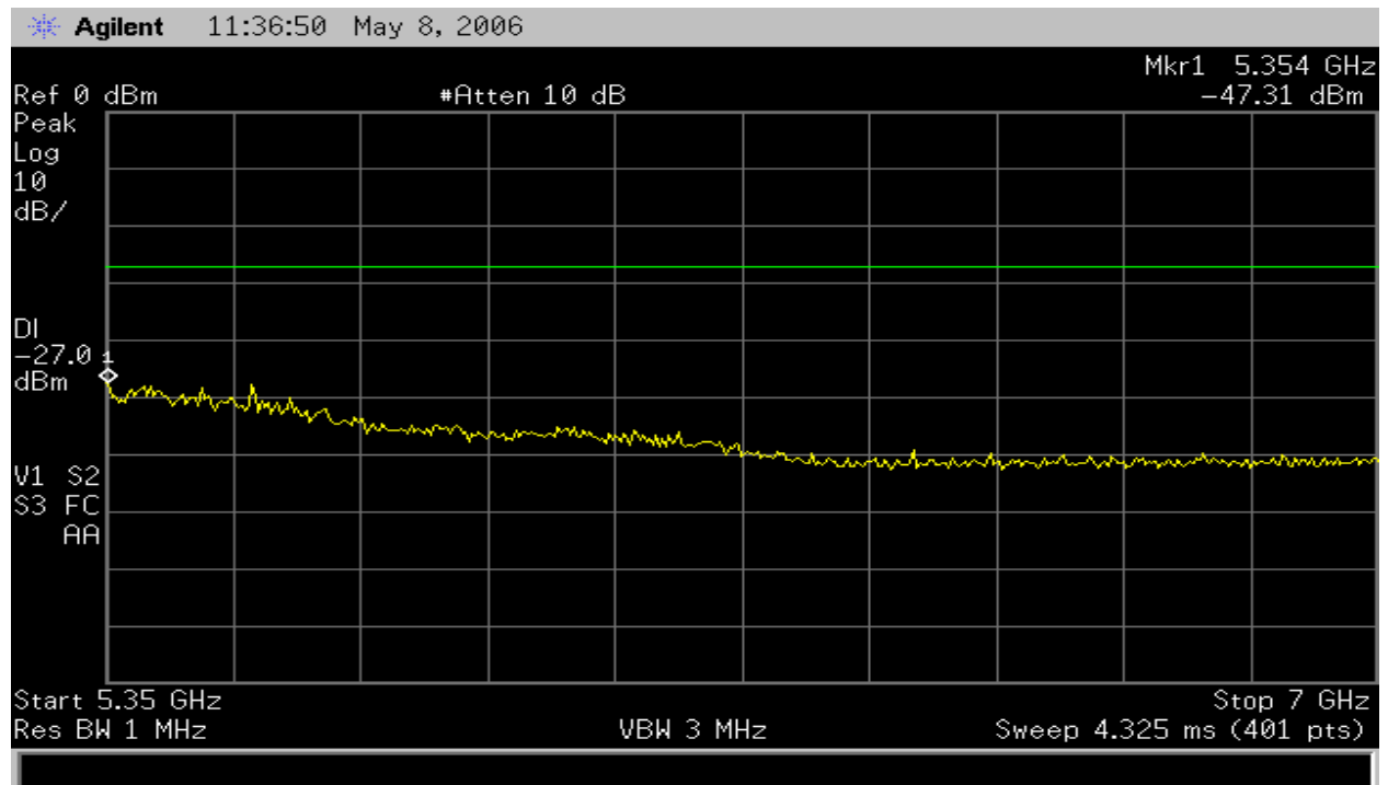
Figure 19 – 802.11a Conducted Spurious emissions worst case at 5.18GHz Transmit frequency
