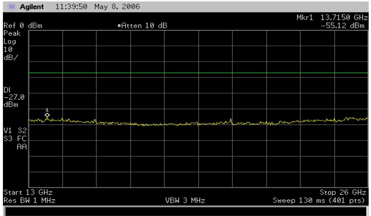
Figure 21 – 802.11a Conducted Spurious emissions worst case at 5.18GHz Transmit frequency
