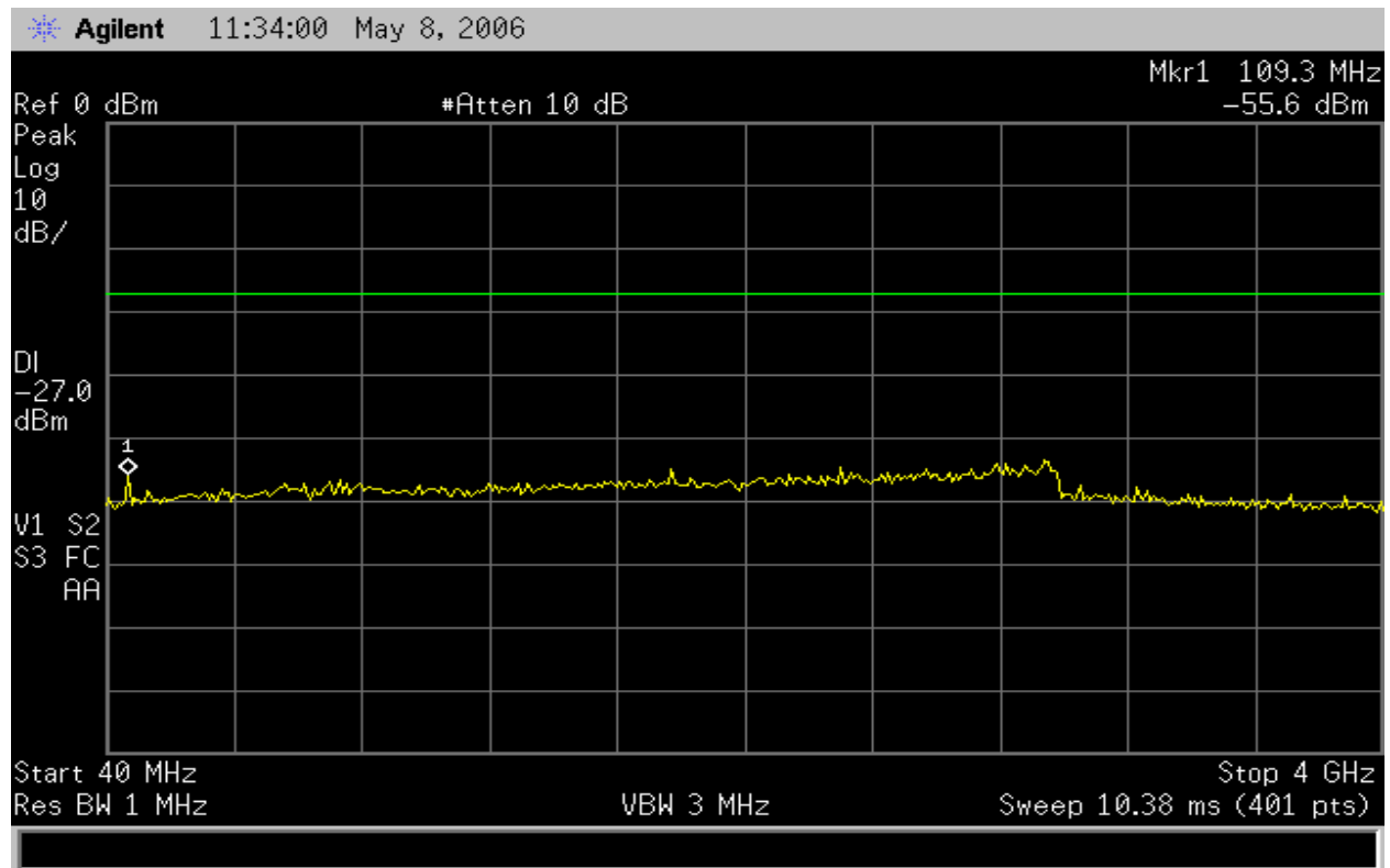
Figure 17 – 802.11a Conducted Spurious emissions worst case at 5.18GHz Transmit frequency
