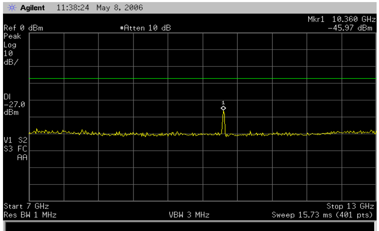
Figure 20 – 802.11a Conducted Spurious emissions worst case at 5.18GHz Transmit frequency
