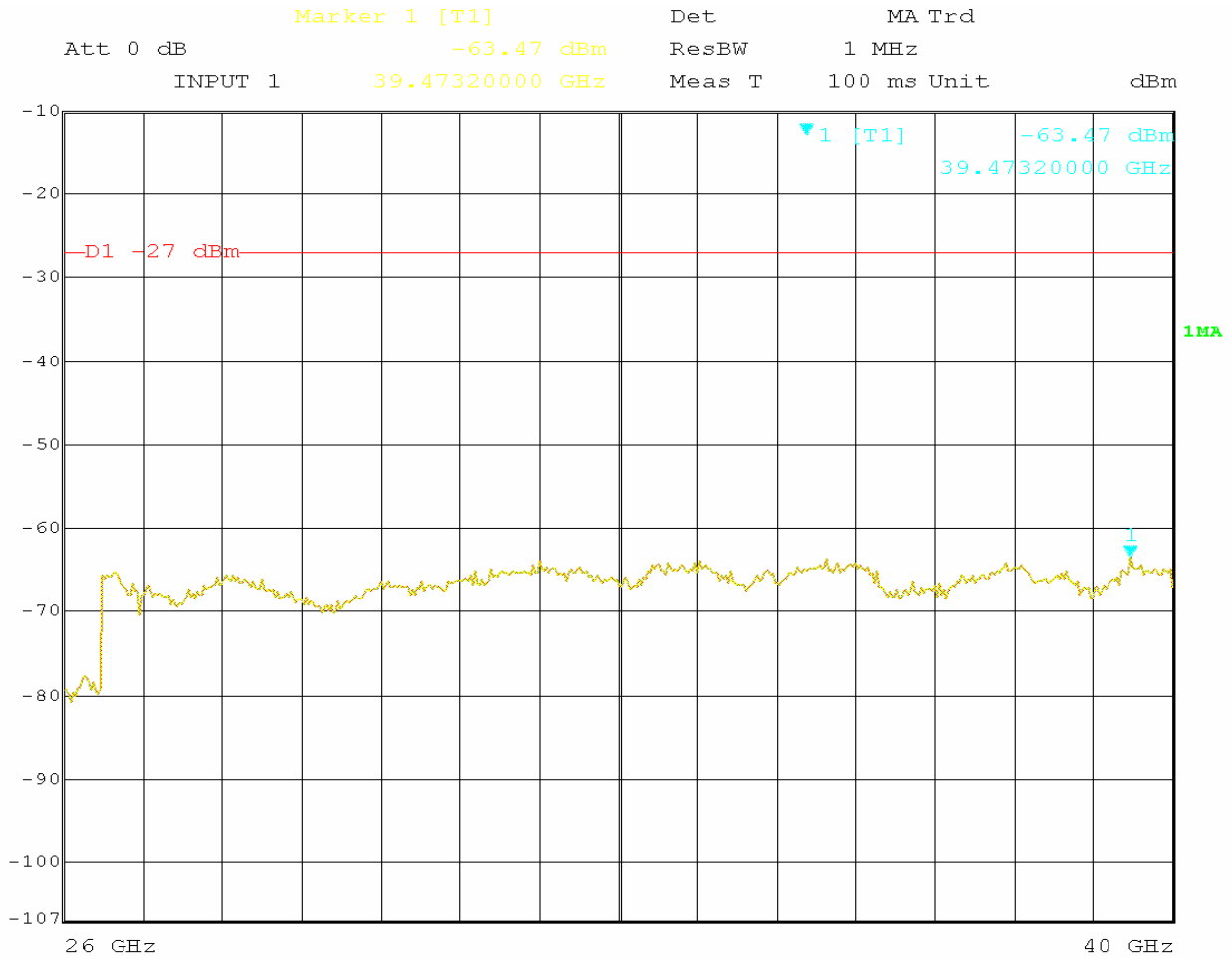
Figure 22 – 802.11a Conducted Spurious emissions worst case at 5.18GHz Transmit frequency
