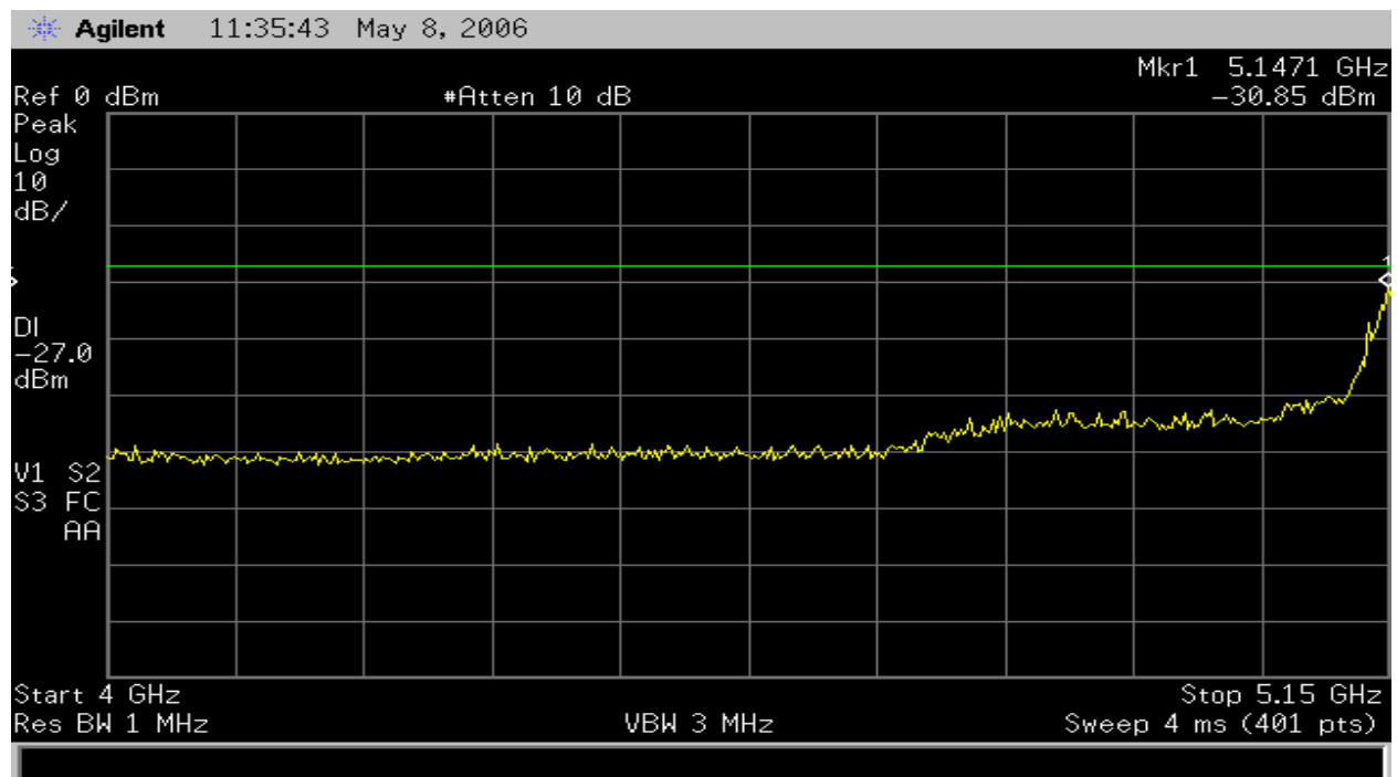
Figure 18 – 802.11a Conducted Spurious emissions worst case at 5.18GHz Transmit frequency
