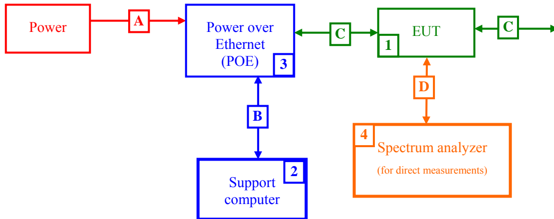
Figure 25 - Block Diagram of EUT Set-Up
