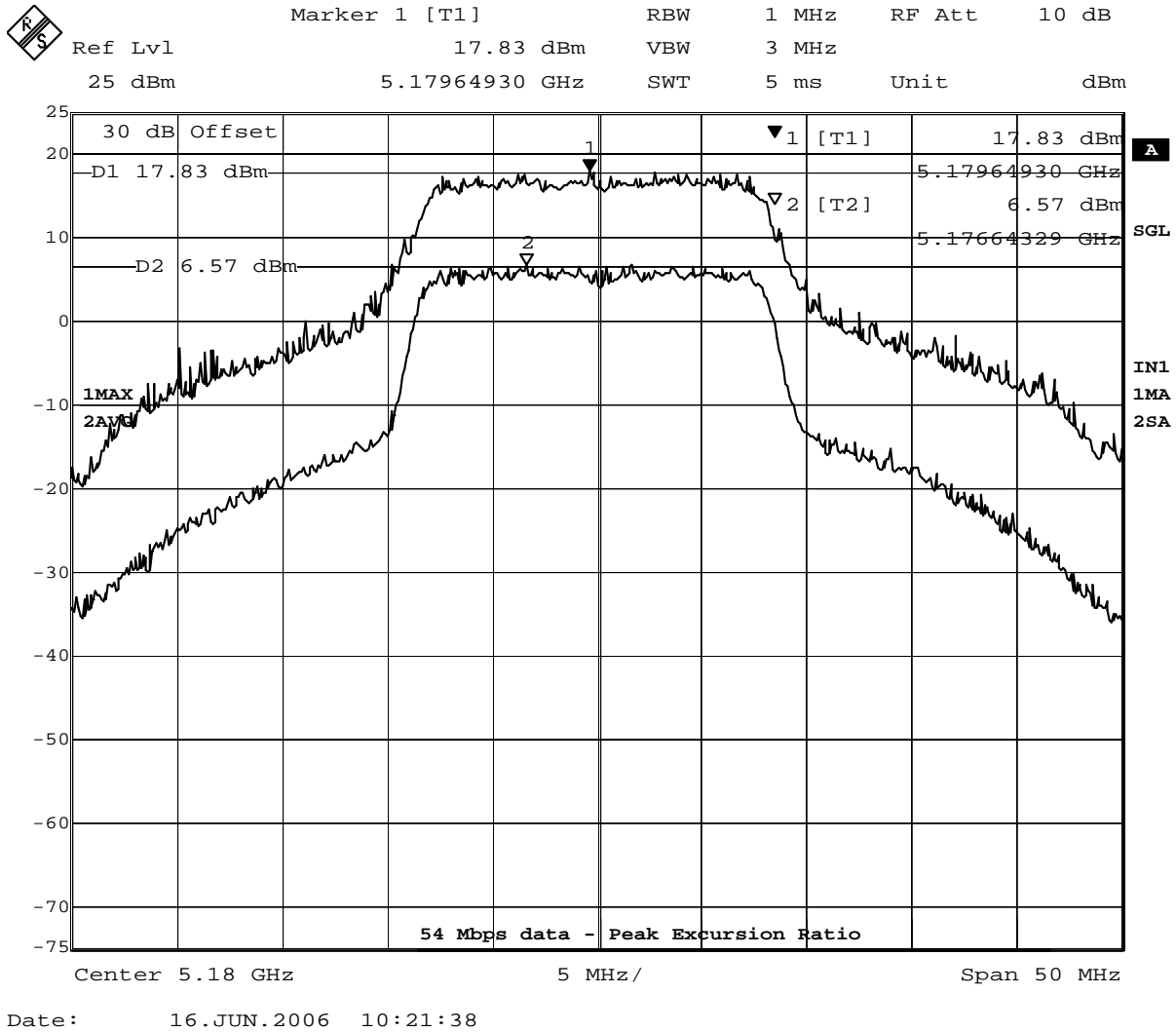
Figure 14 – 802.11a Peak Excursion Ratio; 5.15 – 5.24 GHz band
