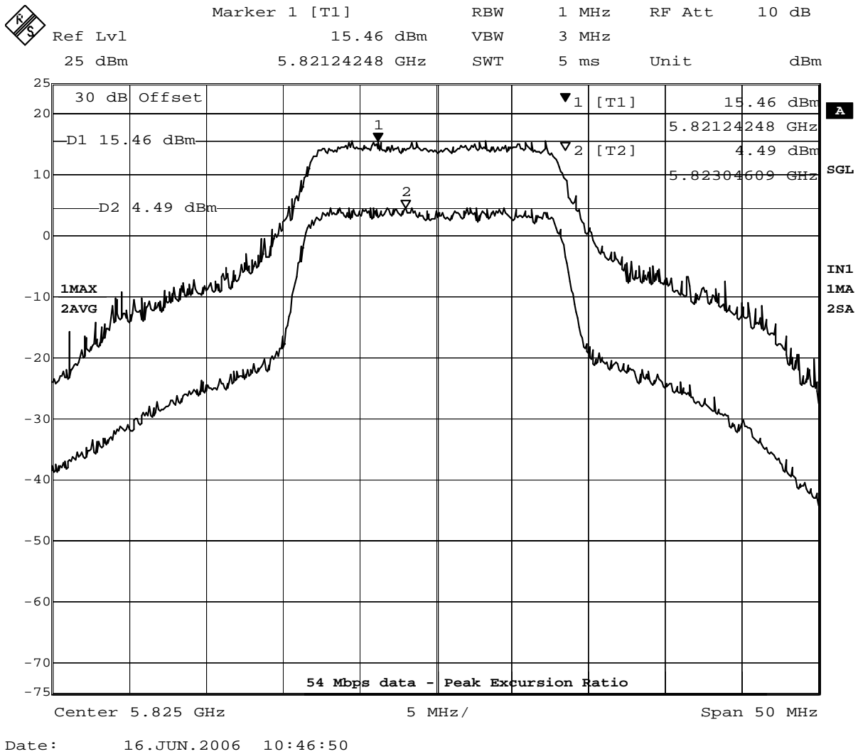
Figure 16 – 802.11a Peak Excursion Ratio; 5.725 – 5.825 GHz band
