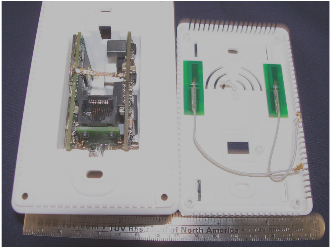
Figure 1 – Internal view of electronics and antennas
