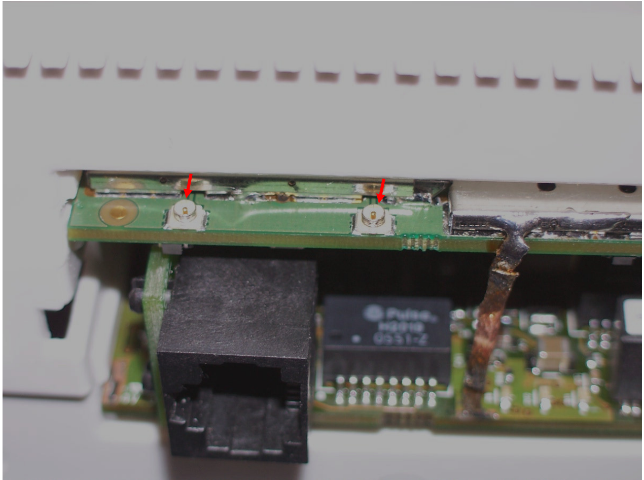
Figure 5 – View of antenna connections on PCB
