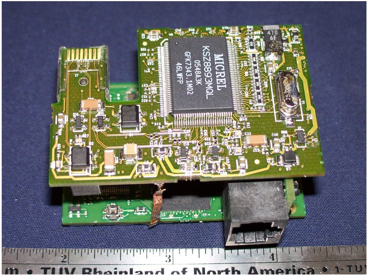
Figure 2 – View of electronic stack
