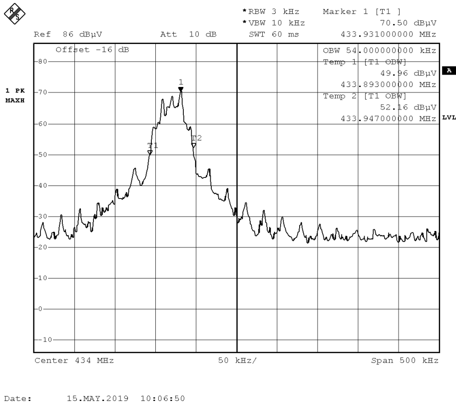
Figure 2: 99% Occupied Bandwidth
