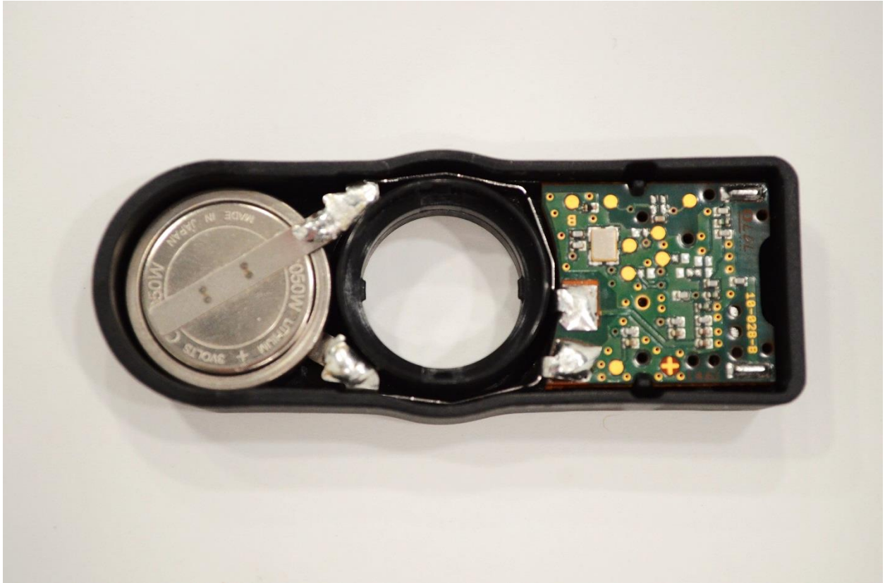
PWB Top
