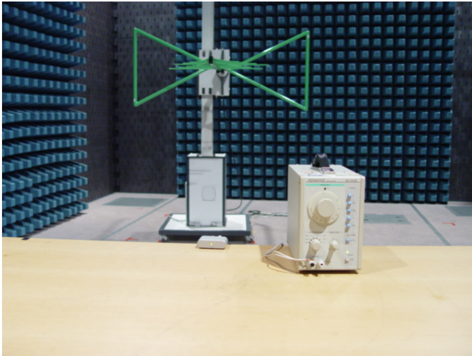
Photo 4 Front View of Radiated Emission Test
