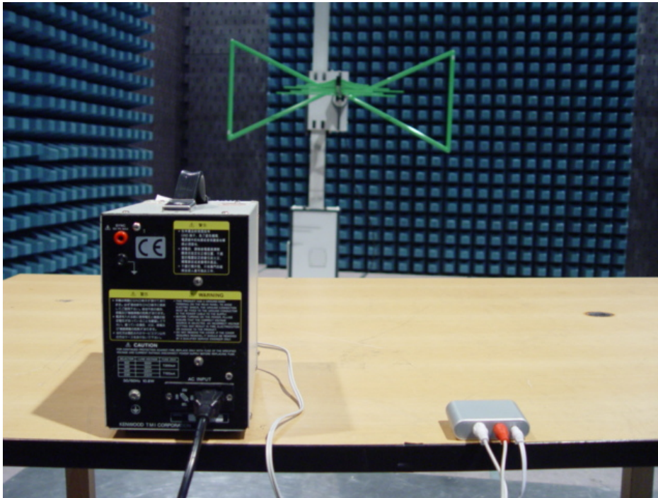
Photo 6 Rear View of Radiated Emission Test
