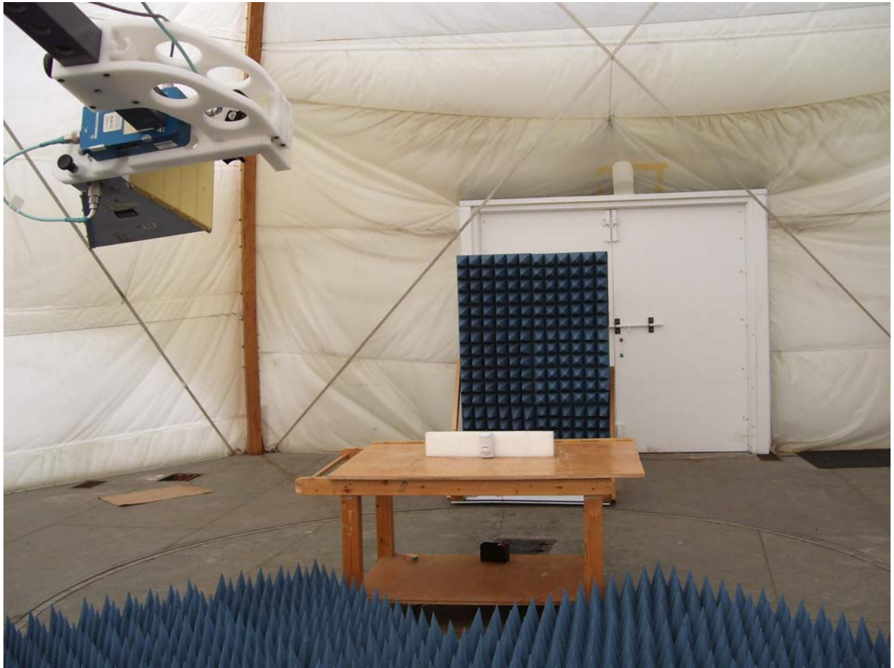
Figure 3: Test Setup View – O.A.T.S above 1 GHz
