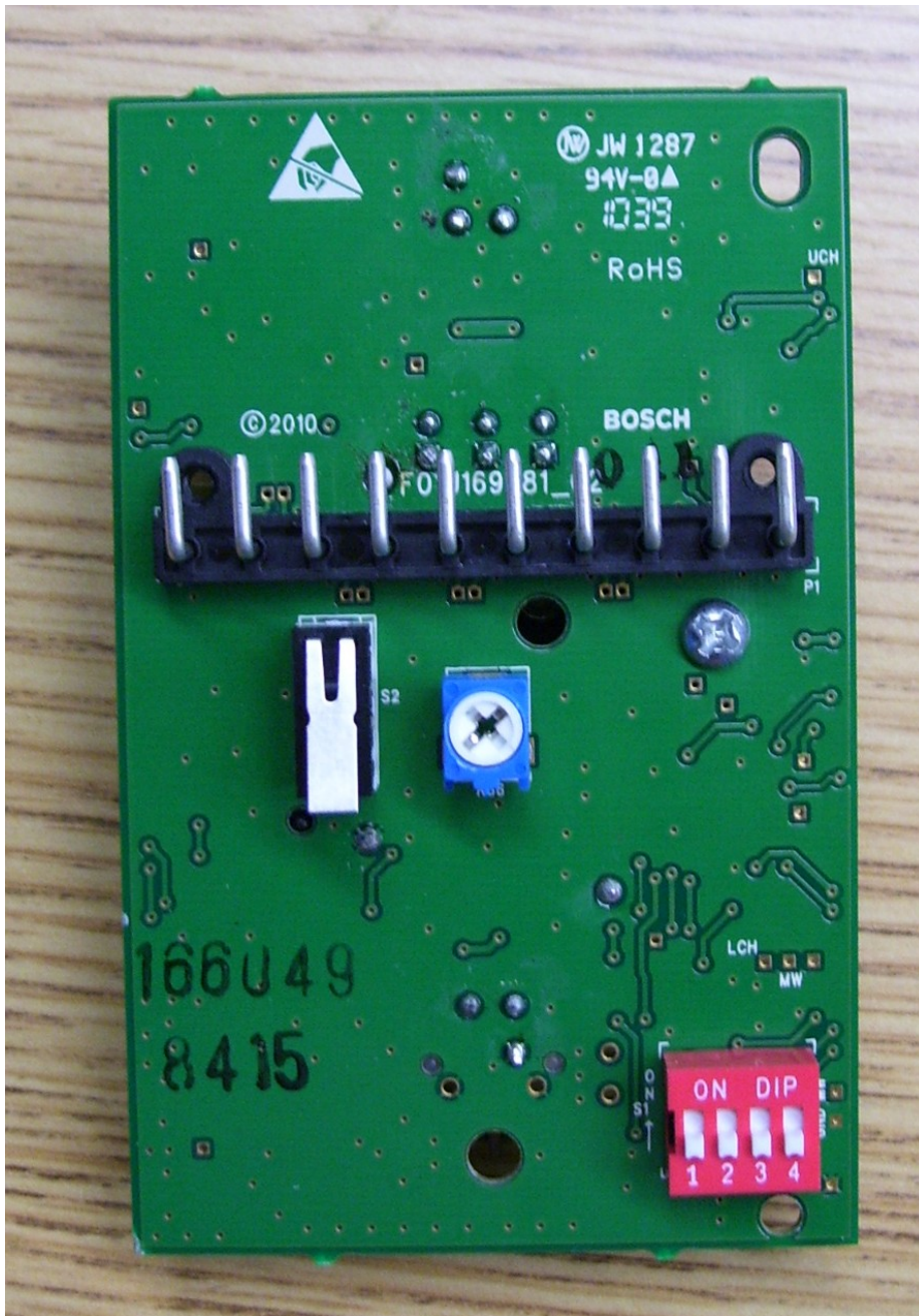
Figure 3: Internal View – Back with Cover Removed
