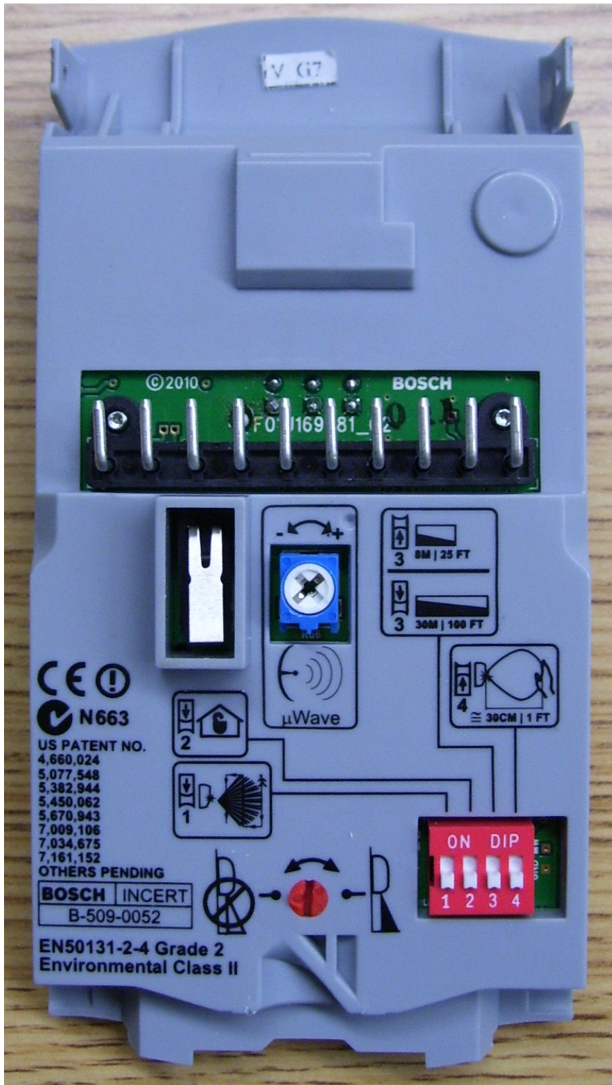
Figure 2: Internal View – Back of Sensor
