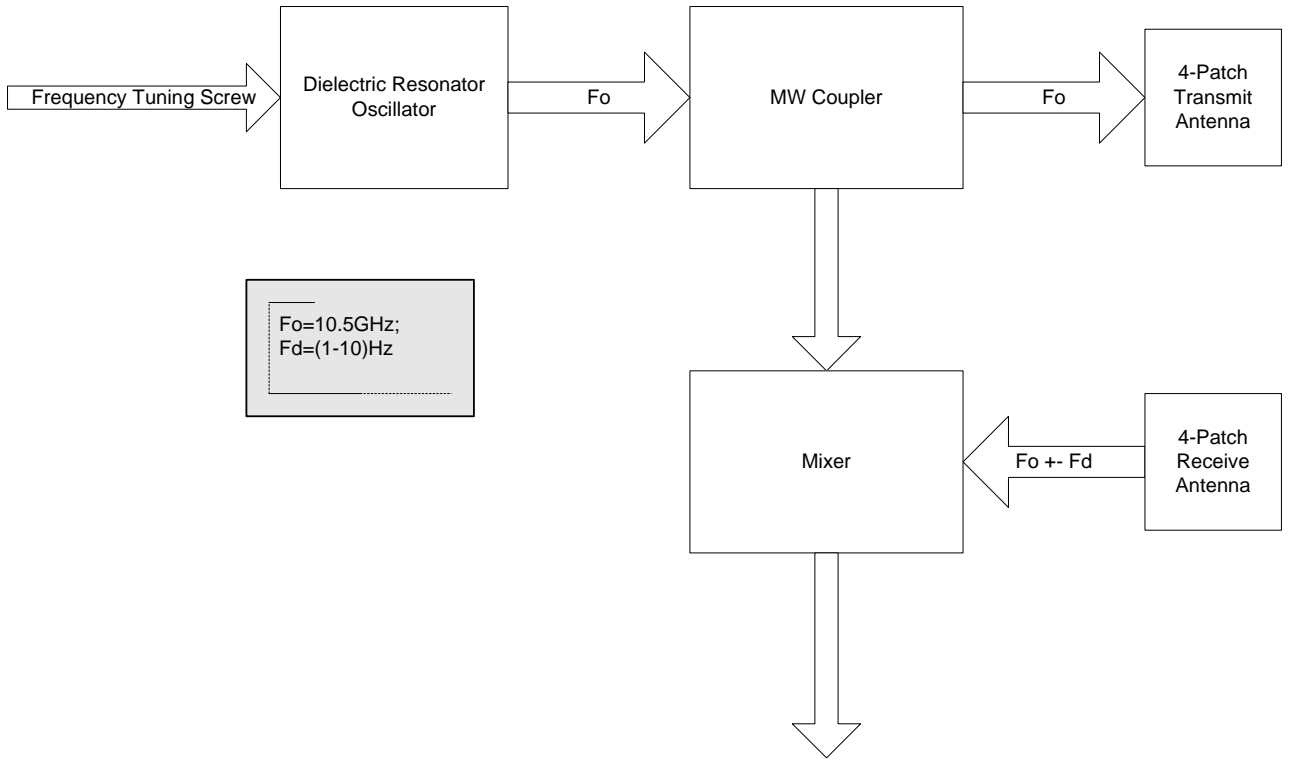
Figure 2: DCSC-G Microwave Module Block Diagram
