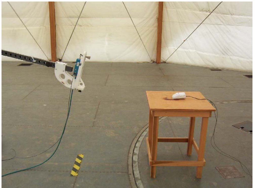
Setup for Spurious emissions on 10 meter OATS – Final test
