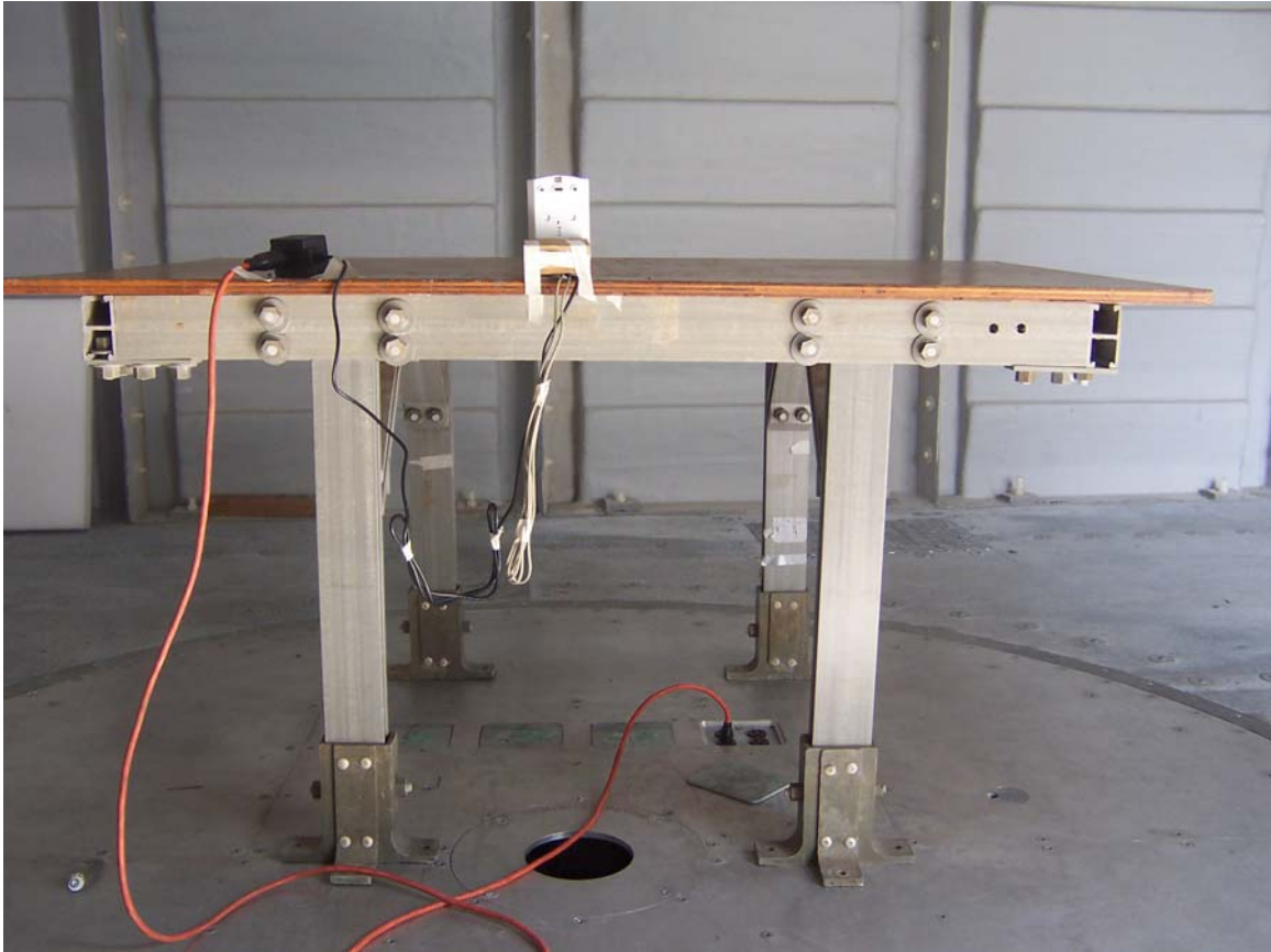
Radiated Emissions Test setup Z-Axis – Back
