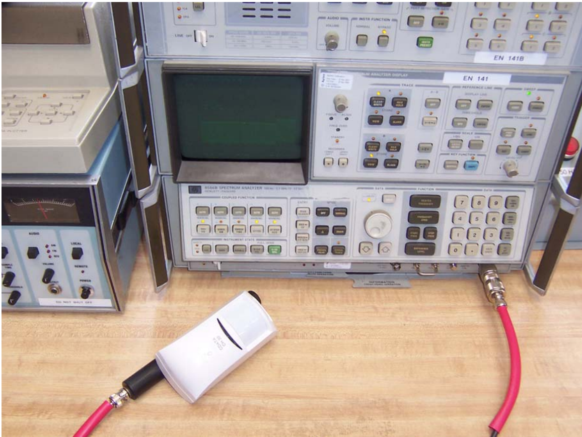
BW, Occupancy Time, 20 dB BW, Carrier frequency separation Test Setup
