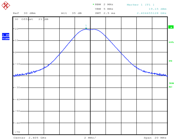
Figure 8.2-1: Conducted output power (2405 MHz)
