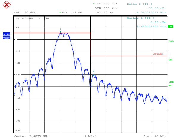
Figure 8.3-8: Upper band edge, Conducted (TX 2480 MHz) @ -14 dBm
