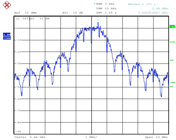
Figure 8.4-2: PSD (2440 MHz)
