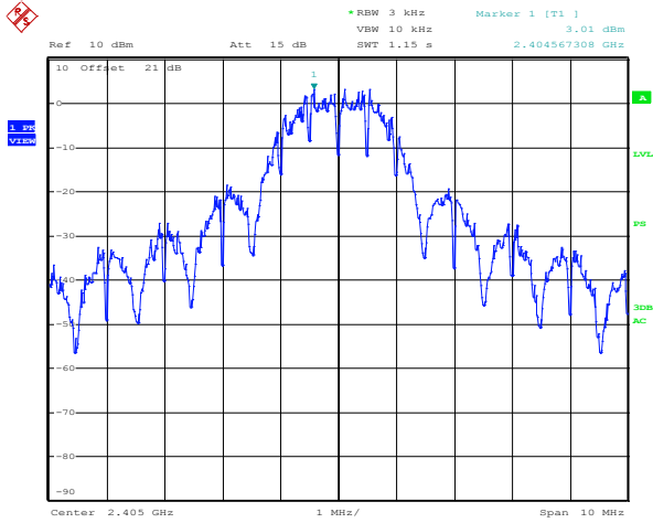
Figure 8.4-1: PSD (2405 MHz)
