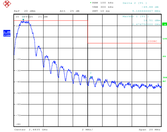
Figure 8.3-7: Upper band edge, Conducted (TX 2475 MHz)
