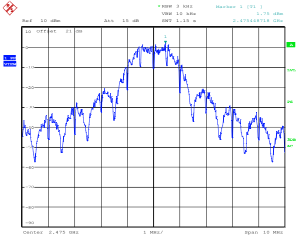
Figure 8.4-3: PSD (2475 MHz)
