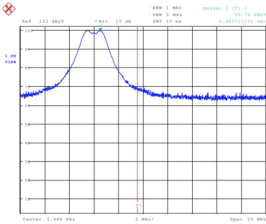
Plot 8.3-18: Upper band edge 1 MHz RBW, 3 MHz VBW, Radiated (TX 2480 MHz) – Circular SEMI-Loop Antenna
