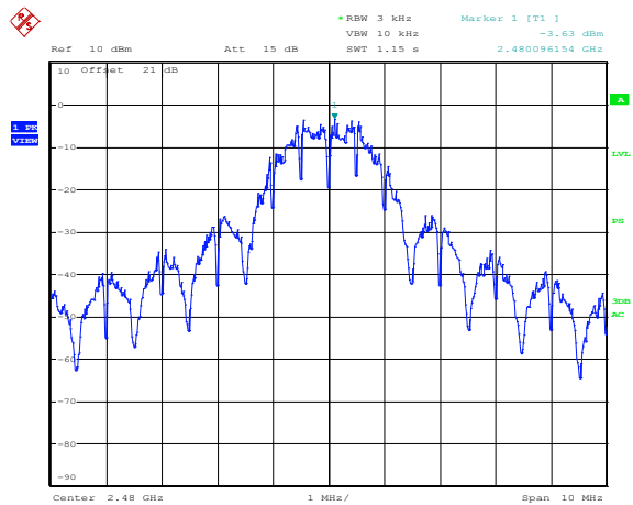
Figure 8.4-4: PSD (2480 MHz) @ -12 dBm
