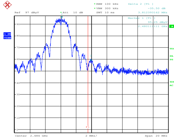
Plot 8.3-19: Upper band edge 100 kHz RBW, 300 kHz VBW, Radiated (TX 2480 MHz) – Circular SEMI-Loop Antenna
