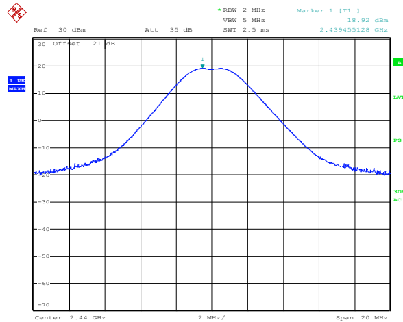
Figure 8.2-2: Conducted output power (2440 MHz)
