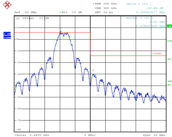
Figure 8.3-9: Upper band edge, Conducted (TX 2480 MHz) @ -12 dBm
