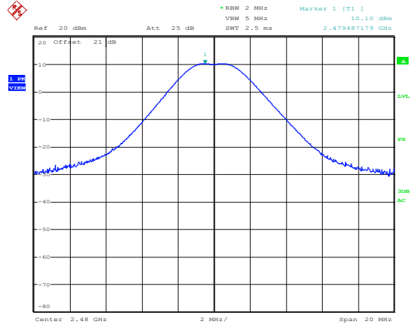
Figure 8.2-4: Conducted output power (2480 MHz) @ -14 dBm
