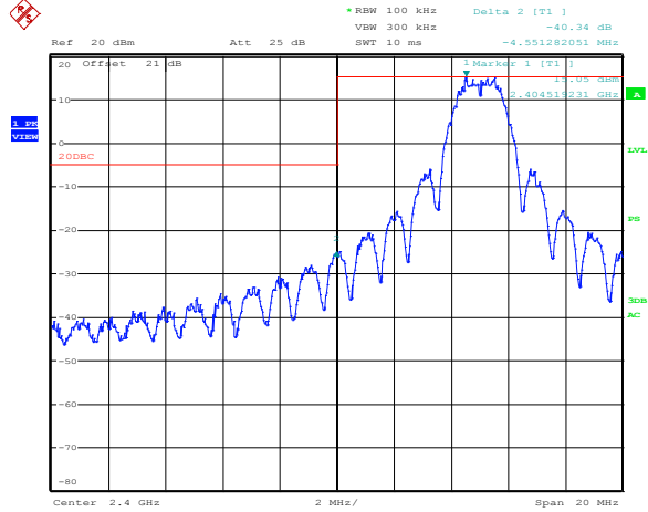
Figure 8.3-6: Lower band edge, Conducted (TX 2405 MHz)
