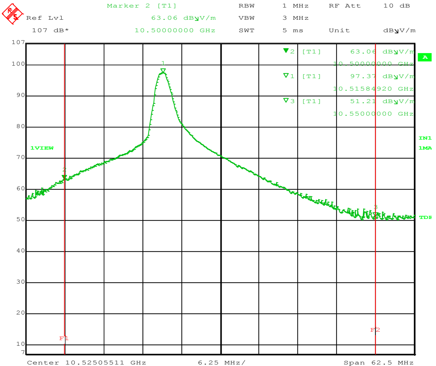
Figure 10 – Band Edge
