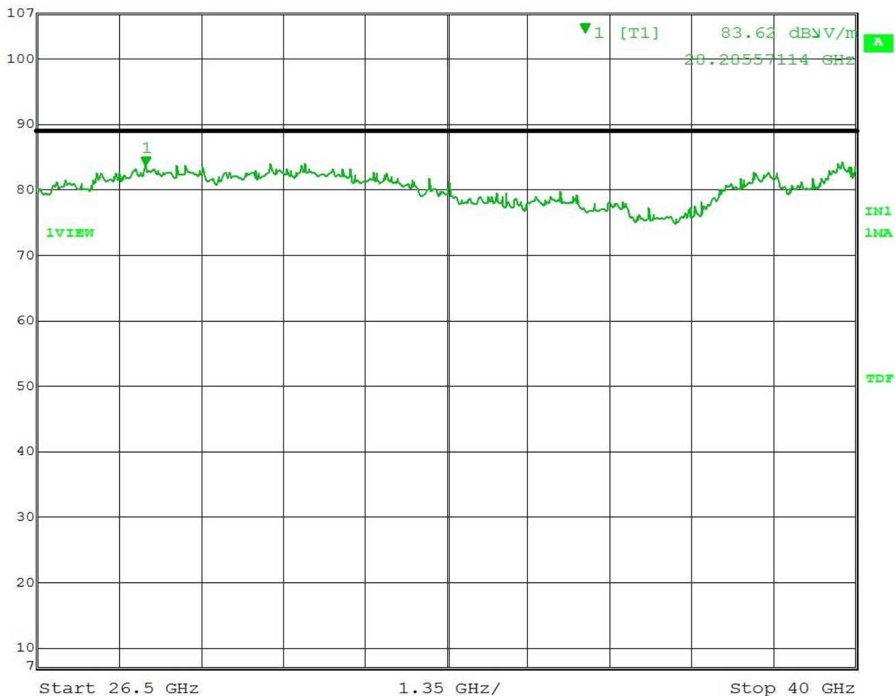
Figure 9 – Field strength of Harmonic Emissions 26.5 - 40 GHz, Vertical
