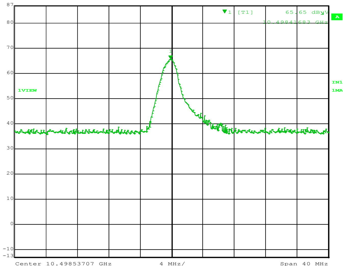
Figure 15 – +55°C Measurement 65.65 dBuV + 21.8db = 87.45 dBuV (Calculated)
