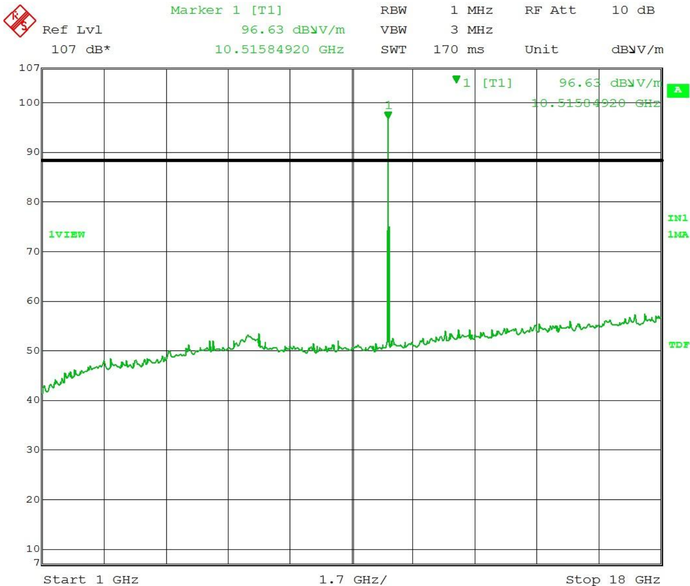
Figure 4 – Field strength of Harmonic Emissions 1-18 GHz, Horizontal
