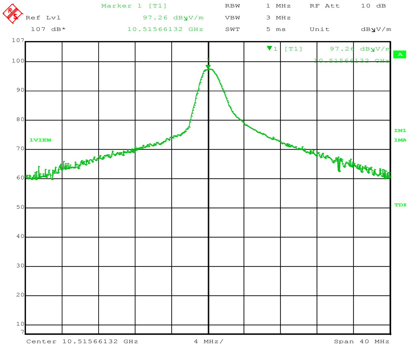
Figure 2 – Horizontal, 97.26 dBuV/m
