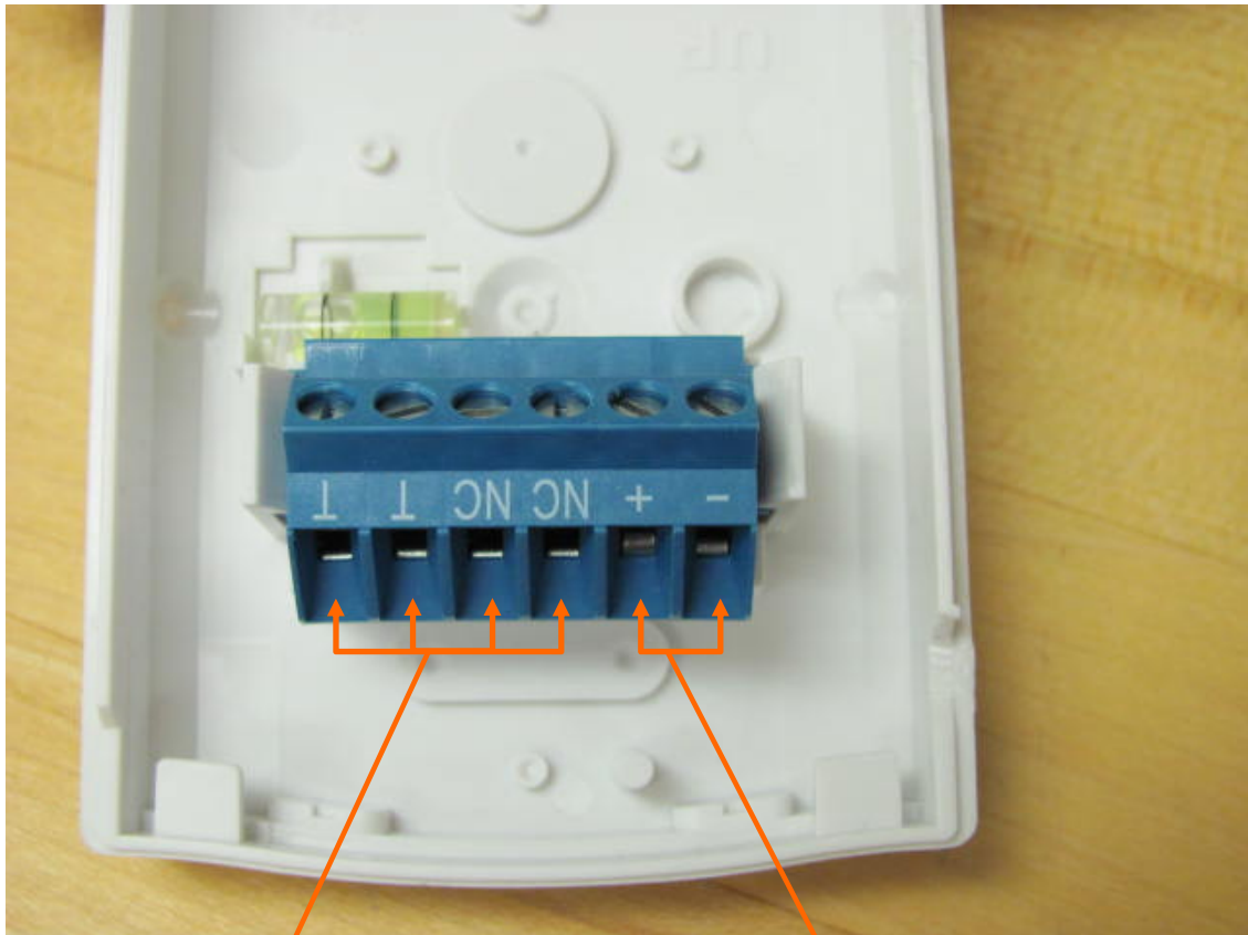
Figure 5: View of Connector assembly.
