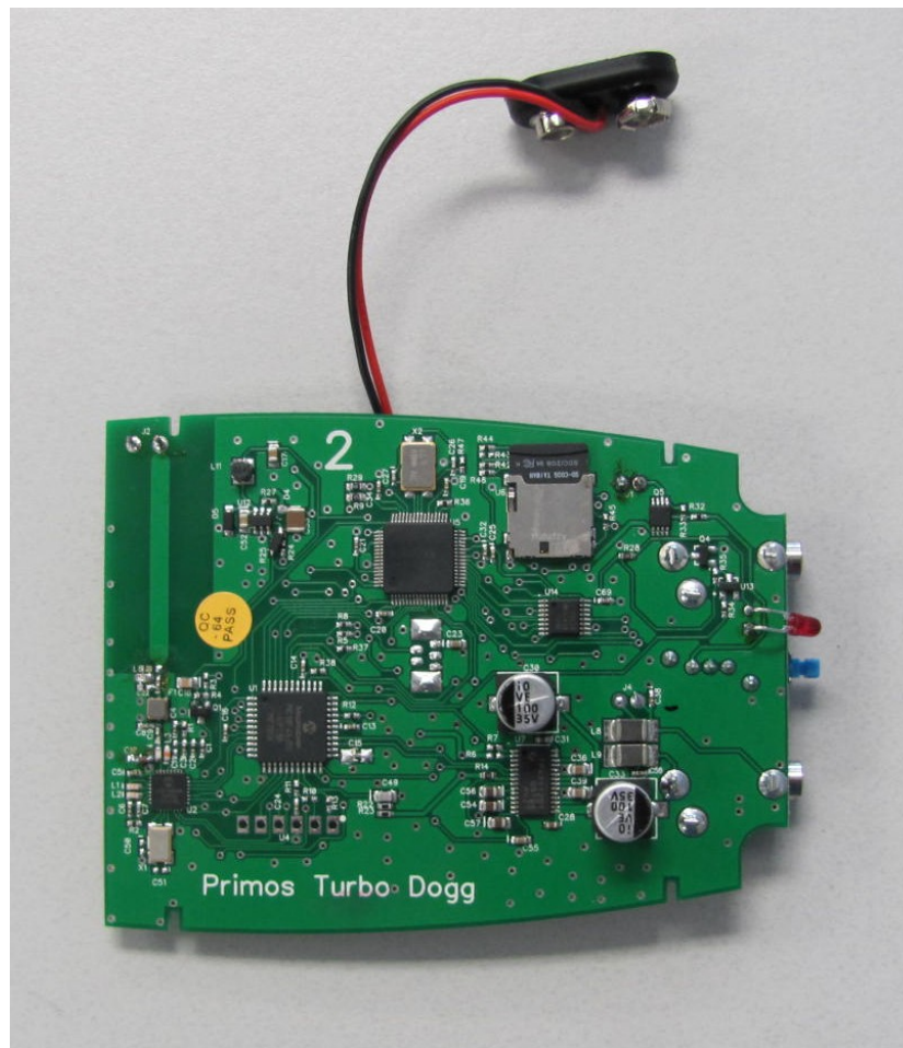
Photograph of Turbo Dogg PC Board: Foil Side
