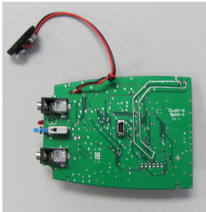
Photograph of Turbo Dogg PC Board: Foil Side
