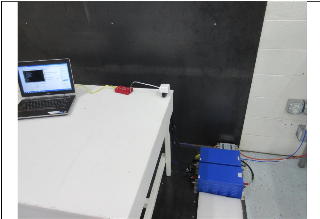
AC Conducted #2
