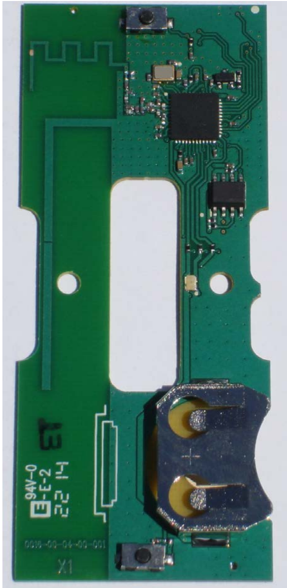
PCB Topside
