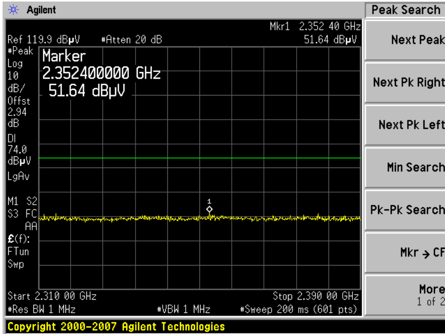
Low Channel – 2405 MHz Horizontal, Peak
