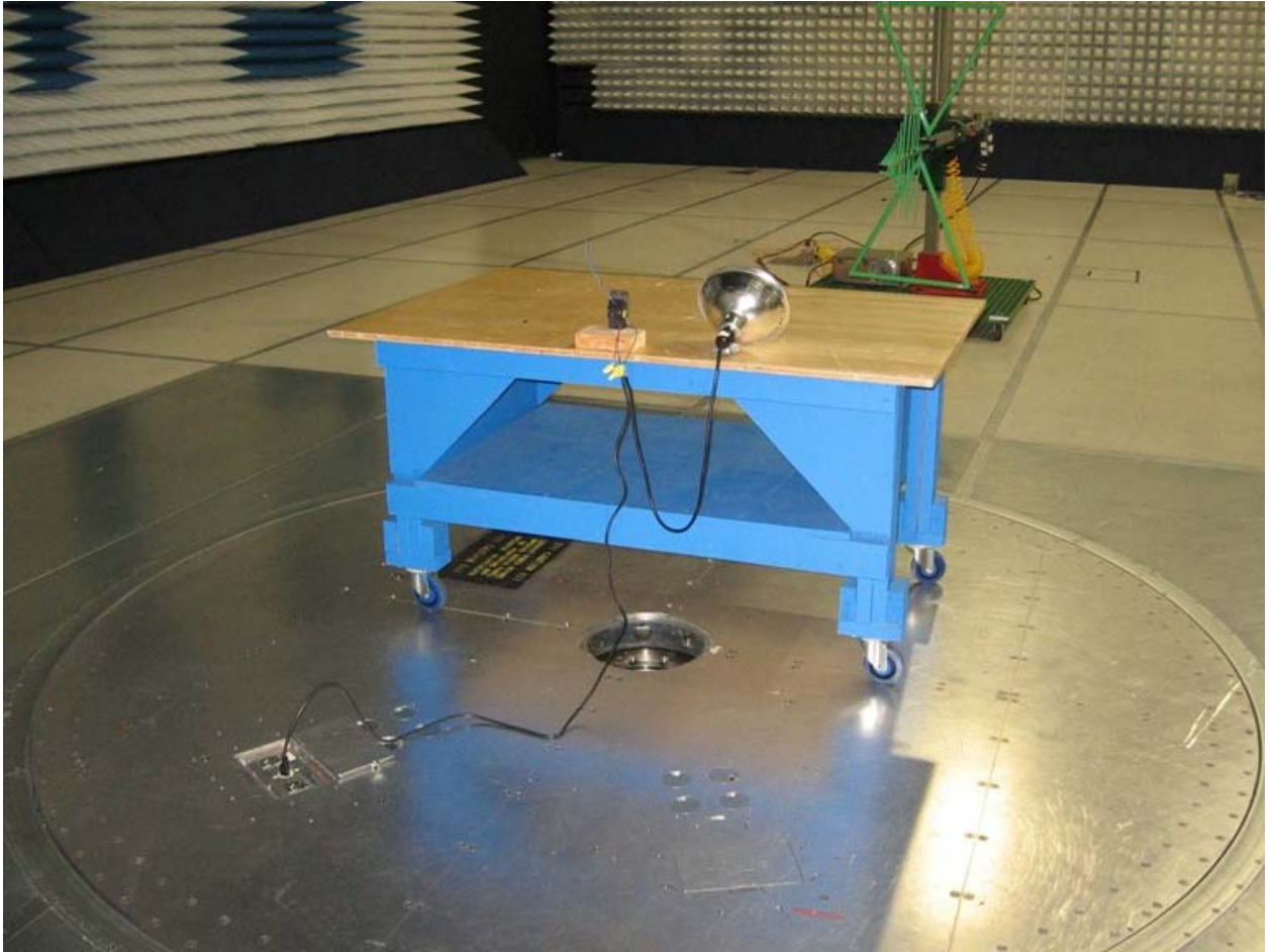
Radiated Emissions – Rear View
