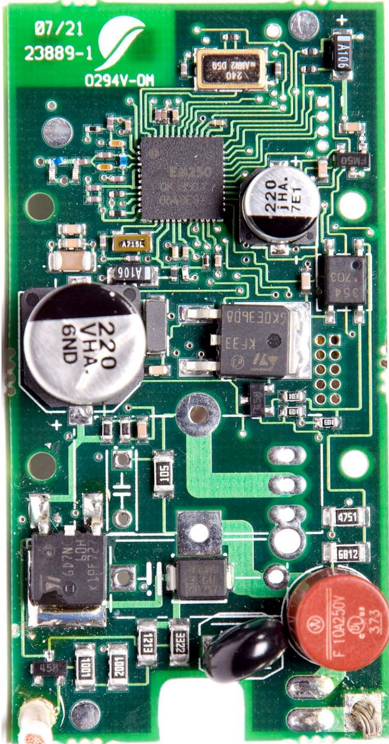
PCB – Bottom View
