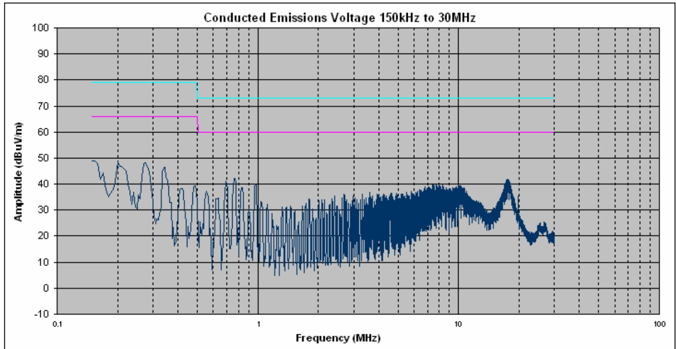
Conducted Emission, Neutral Line Plots
