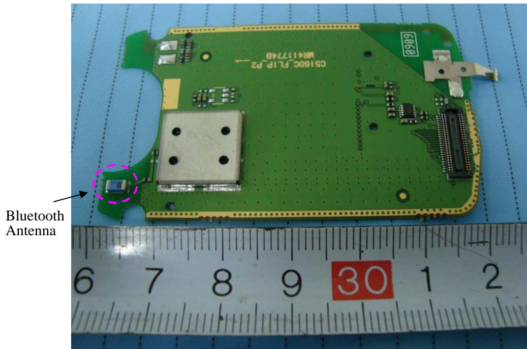
EUT – Flip Board Components View
