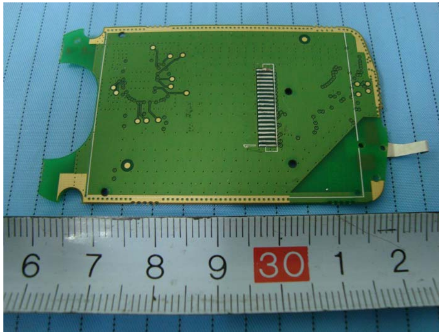
EUT – Flip Board Circuit View
