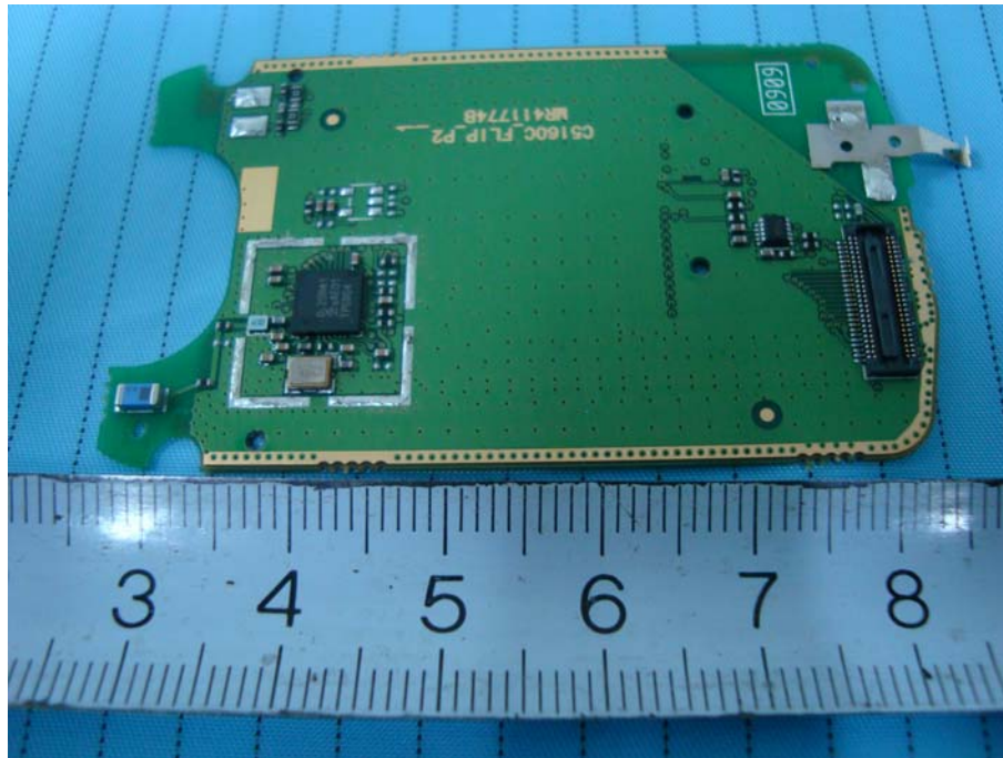
EUT – Flip Board With Shielded-Cover Components View
