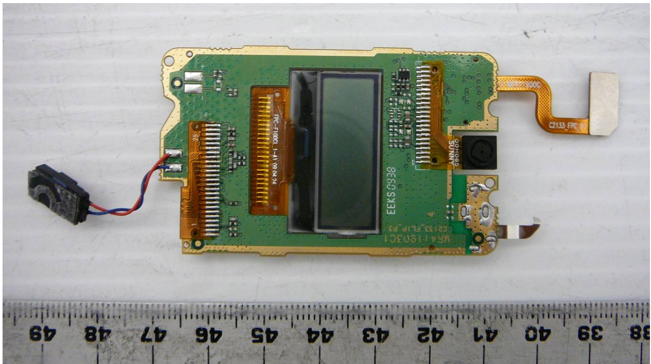
EUT Internal – LCD Board Assembly Bottom View
