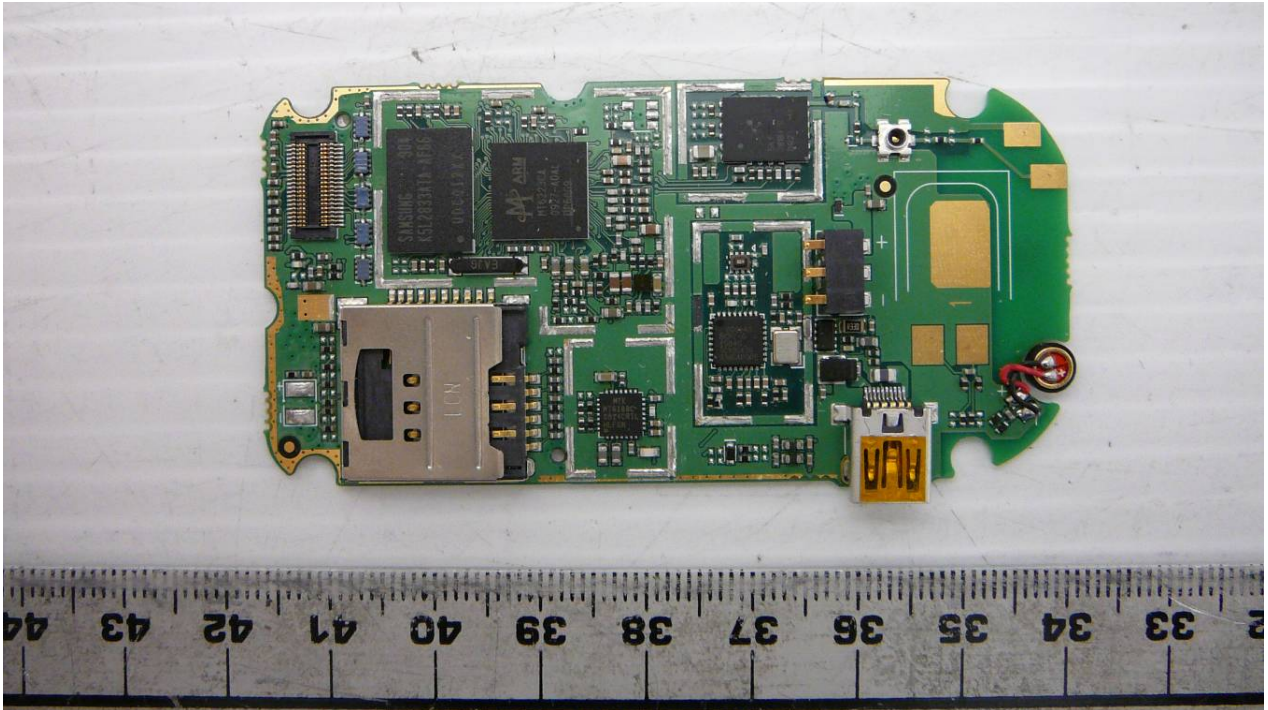
EUT Internal – Board Assembly Bottom (Antenna and RF Shielding removed) View
