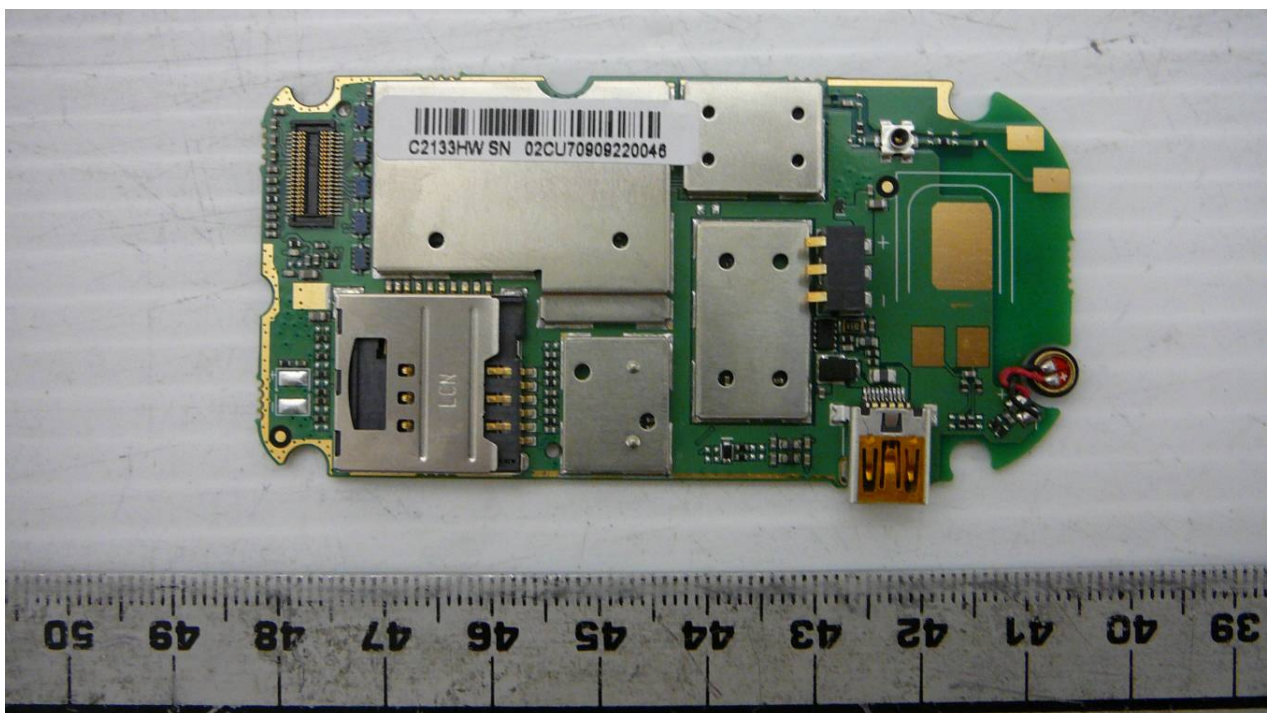
EUT Internal – Board Assembly Bottom (with Antenna and RF Sheilding) View
