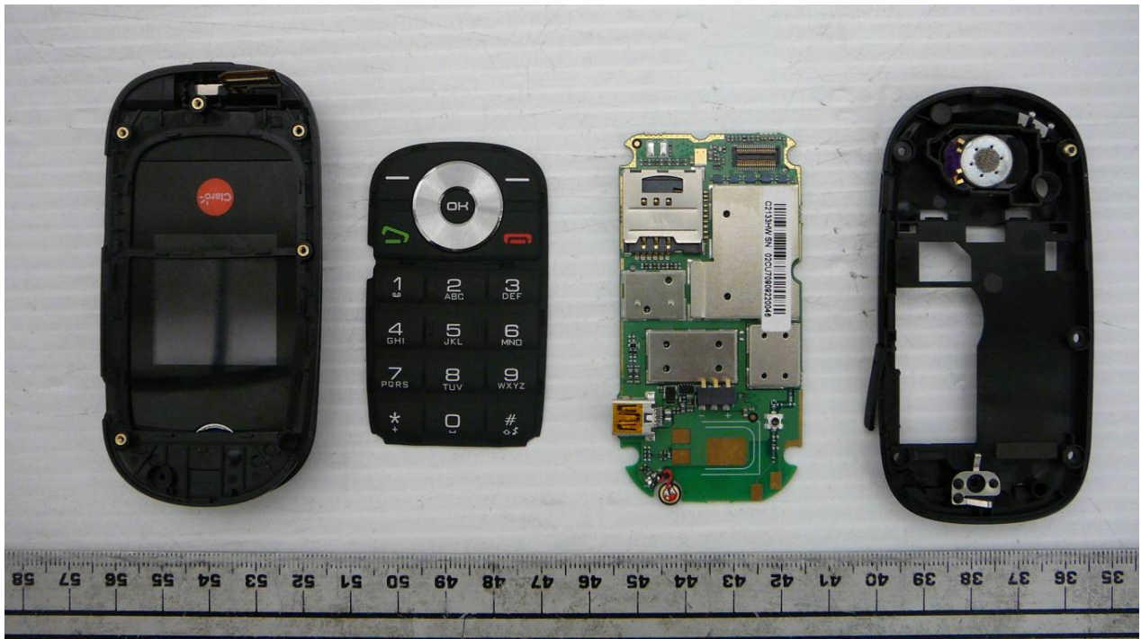
EUT – Battery Compartment View (back cover removed)
