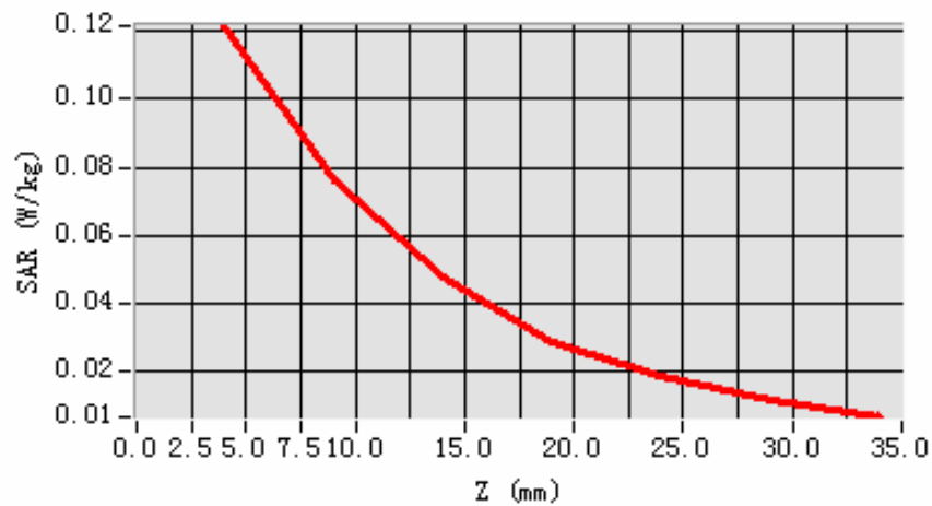
SAR, Z Axis Scan (X = -12, Y = -5)
