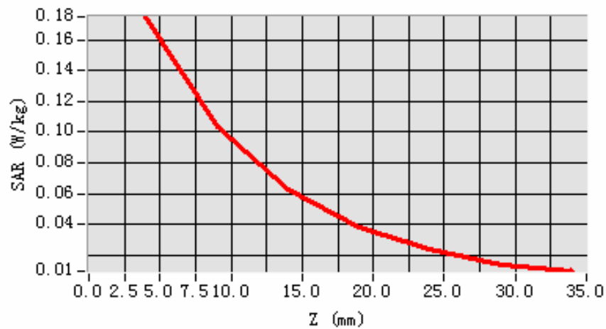
SAR, Z Axis Scan (X = 16, Y = -39)
