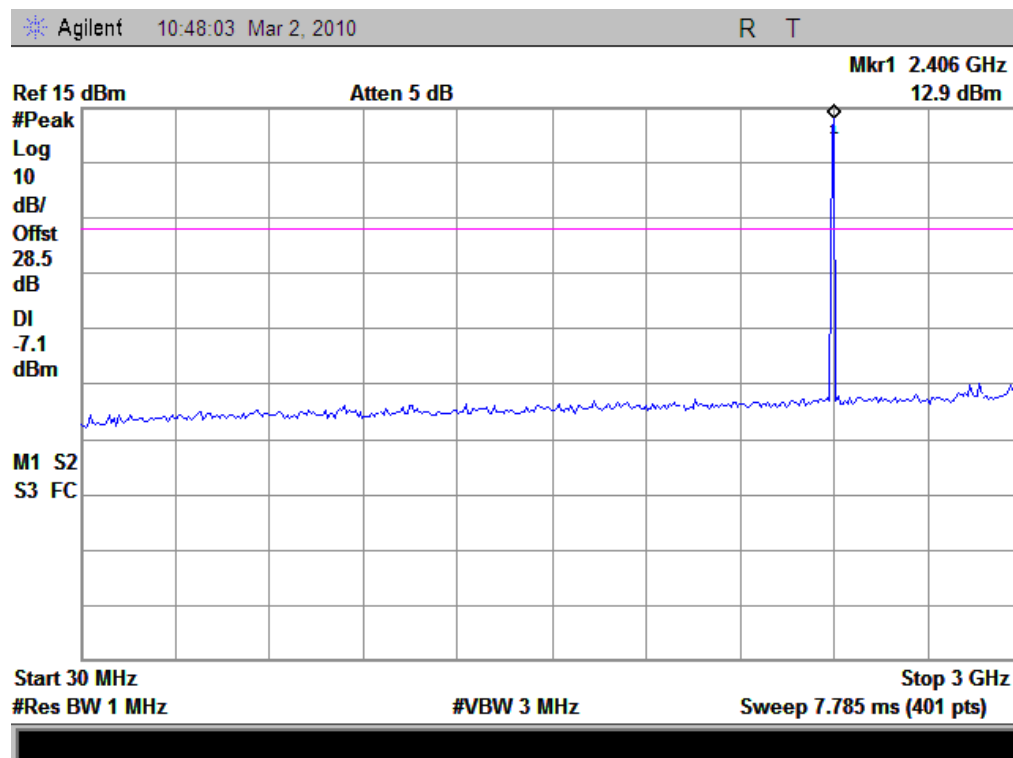
(Plot A.1: Channel = 0, 30MHz to 3GHz)
