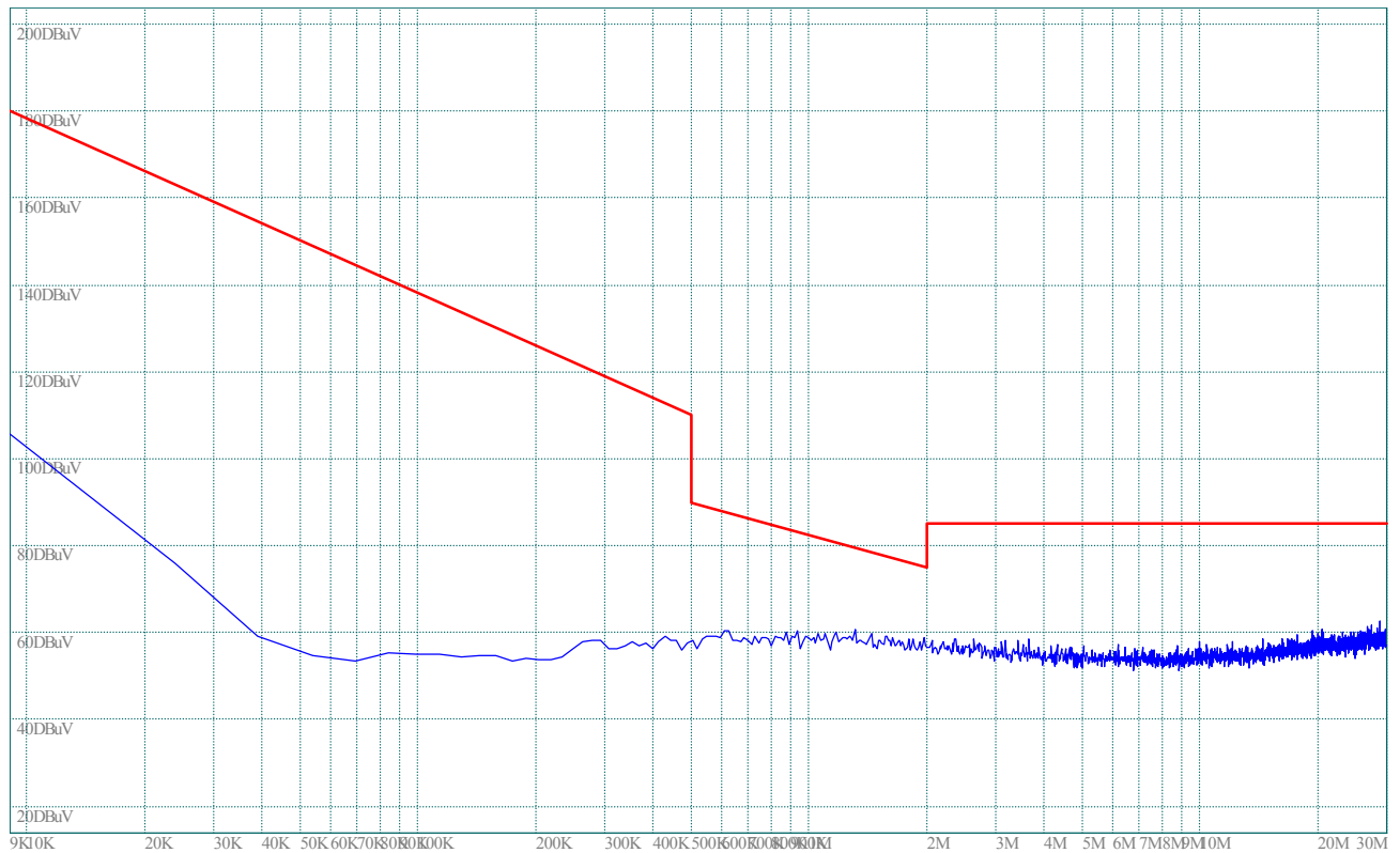
(Plot B.0: 9kHz to 30MHz)
