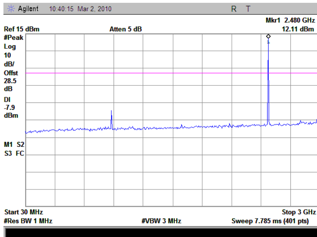
(Plot C.1: Channel = 78, 30MHz to 3GHz)
