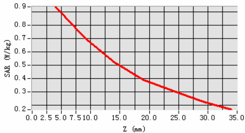
SAR, Z Axis Scan (X = -56, Y = -30)
