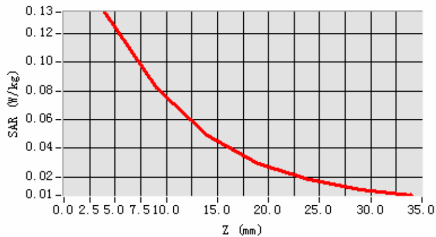
SAR, Z Axis Scan (X = 17, Y = -41)
