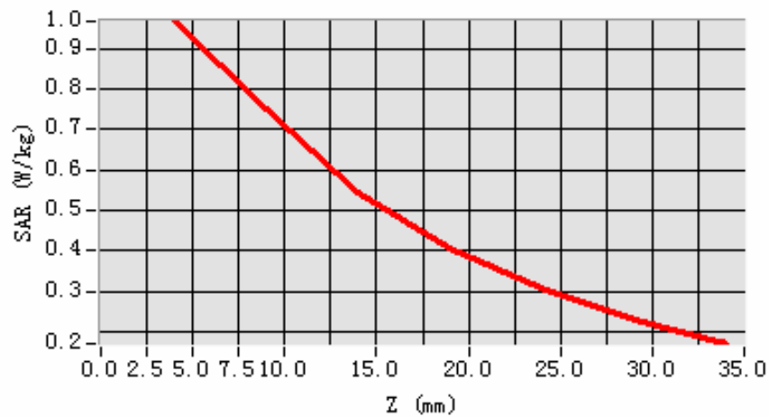
SAR, Z Axis Scan (X = -48, Y = -34)
