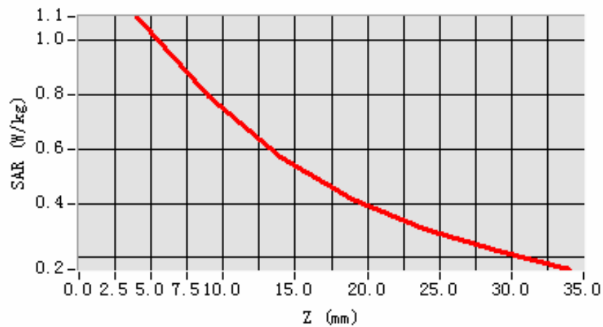
SAR, Z Axis Scan (X = -42, Y = -18)
